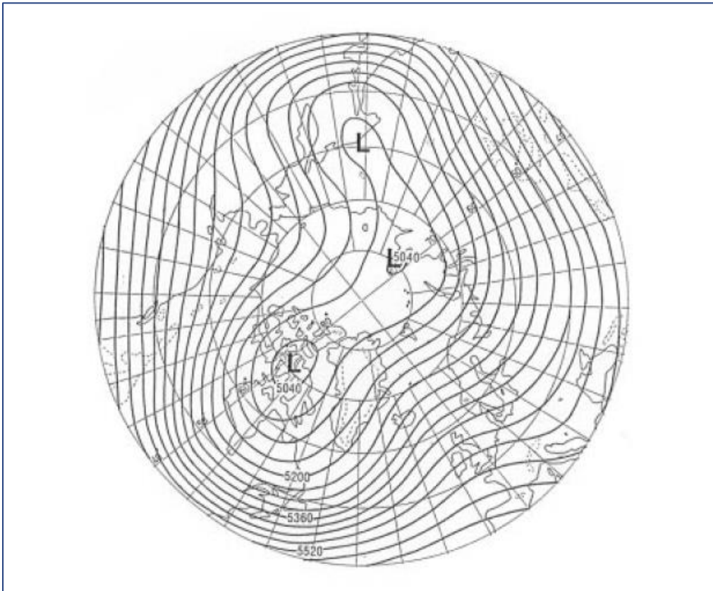
Figure 4. Mean January contour map for the 500 hPa level (altitude stated in metres).
