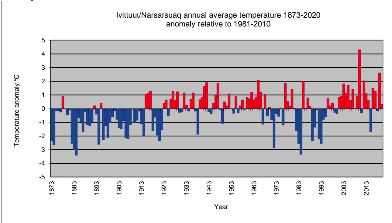
Figure 25. Annual average air temperature since 1873. 34262/4270 Ivittuut/Narsarsuaq, Greenland. Anomaly relative to 1981-2010.
