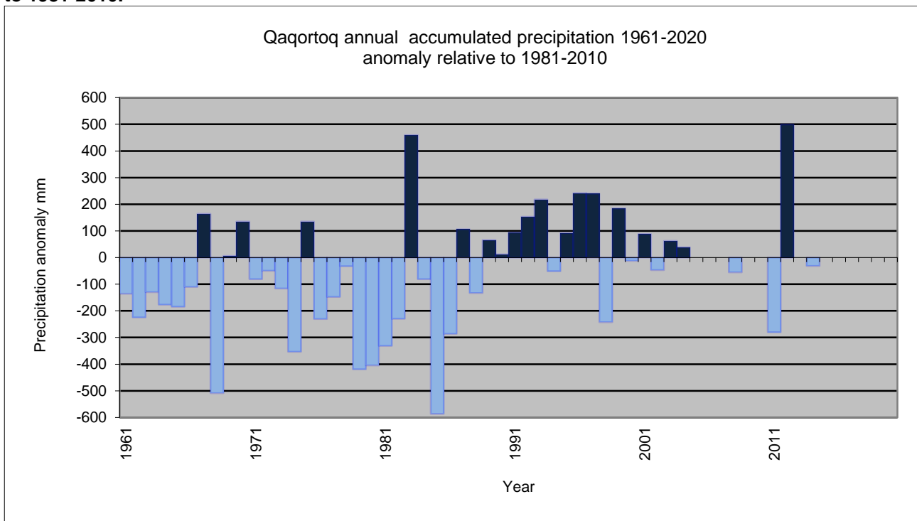
Figure 29. Annual accumulated precipitation since 1961; 4272 Qaqortoq, Greenland. Anomaly relative to 1981-2010.
