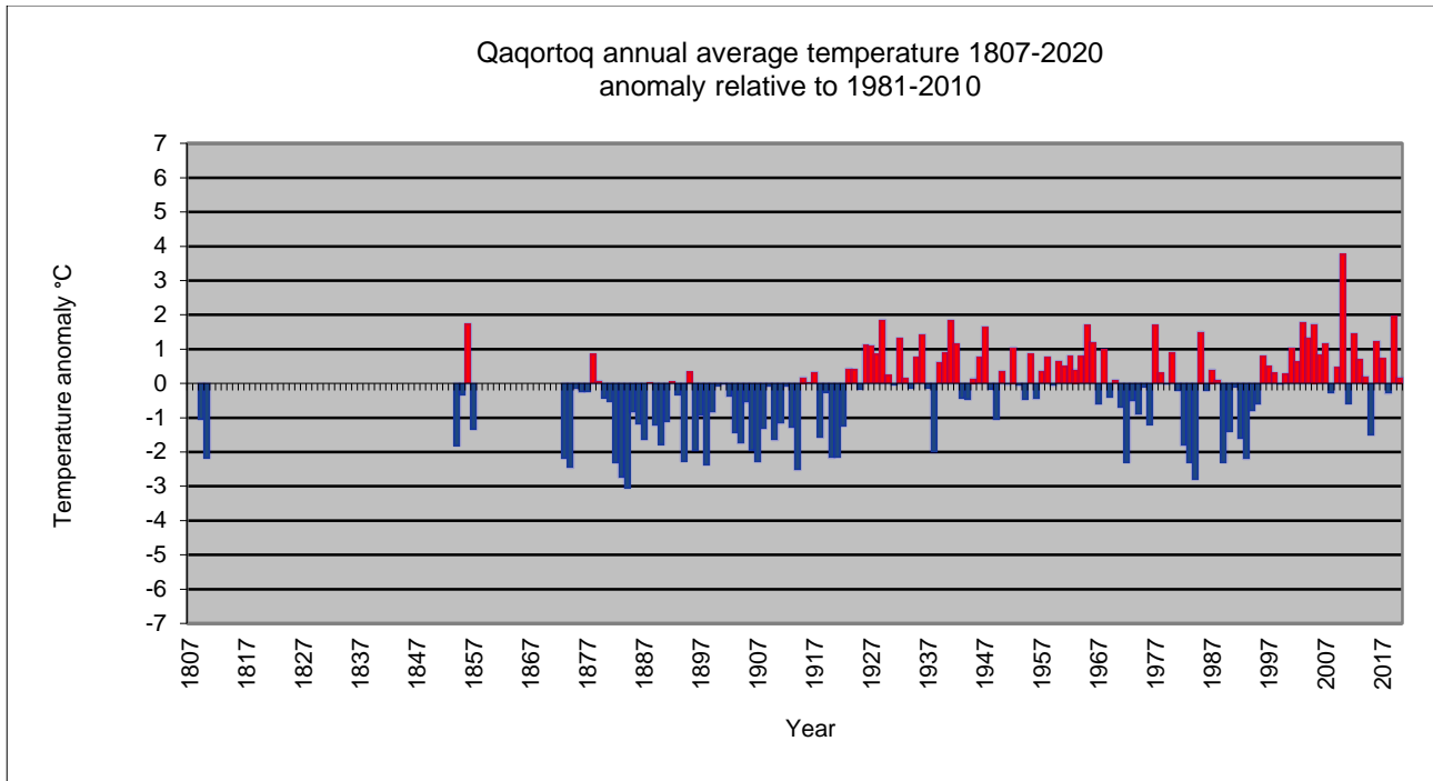
Figure 28. Annual average air temperature since 1807. 4272 Qaqortoq, Greenland. Anomaly relative to 1981-2010.
