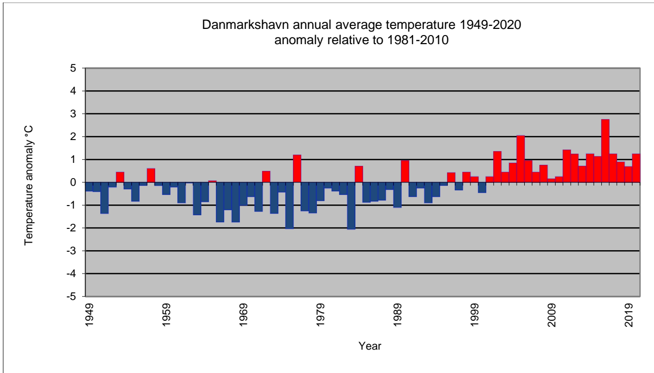
Figure 31. Annual average air temperature since 1949. 4320 Danmarkshavn, Greenland. Anomaly relative to 1981-2010.
