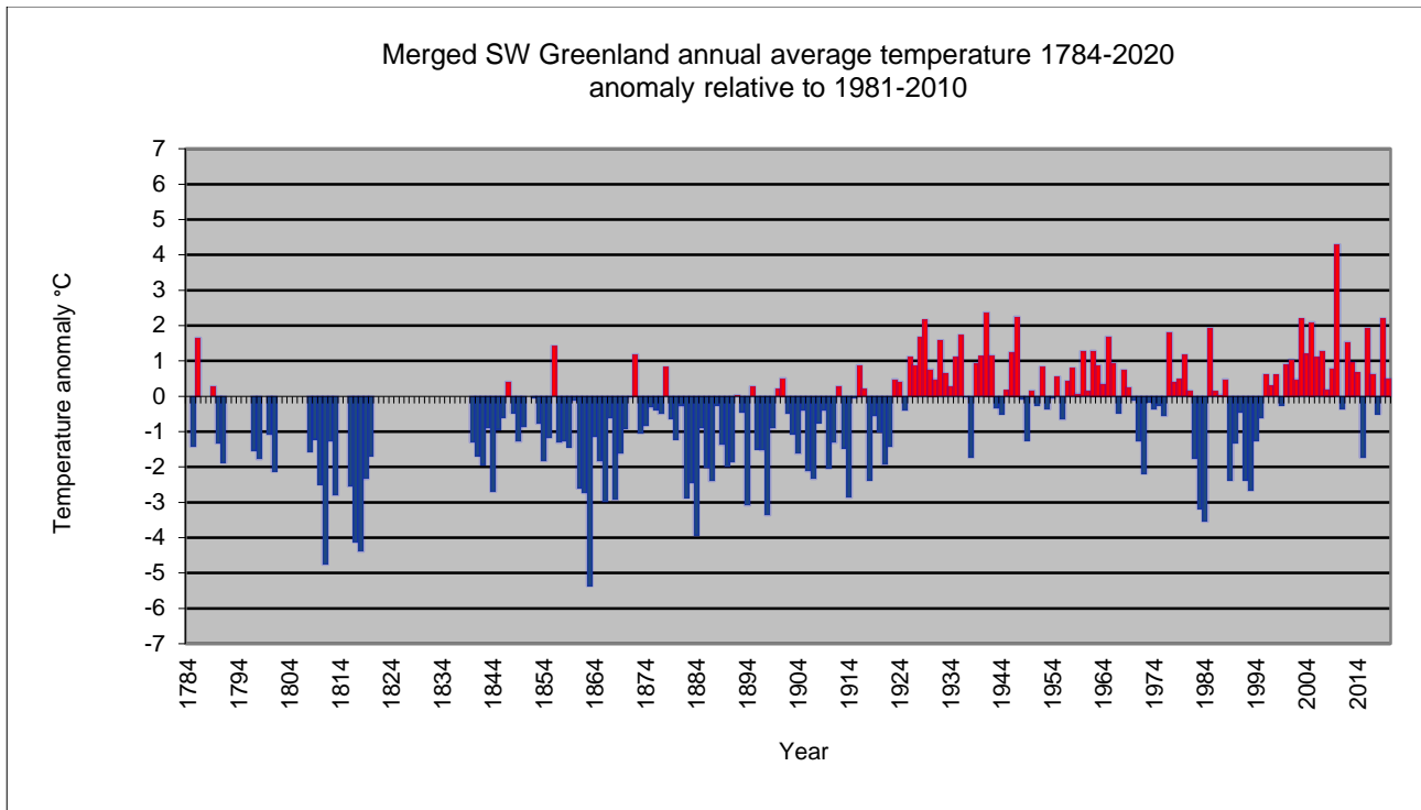
Figure 40. Annual average air temperature since 1784; merged SW Greenland series. Anomaly relative to 1981-2010.
