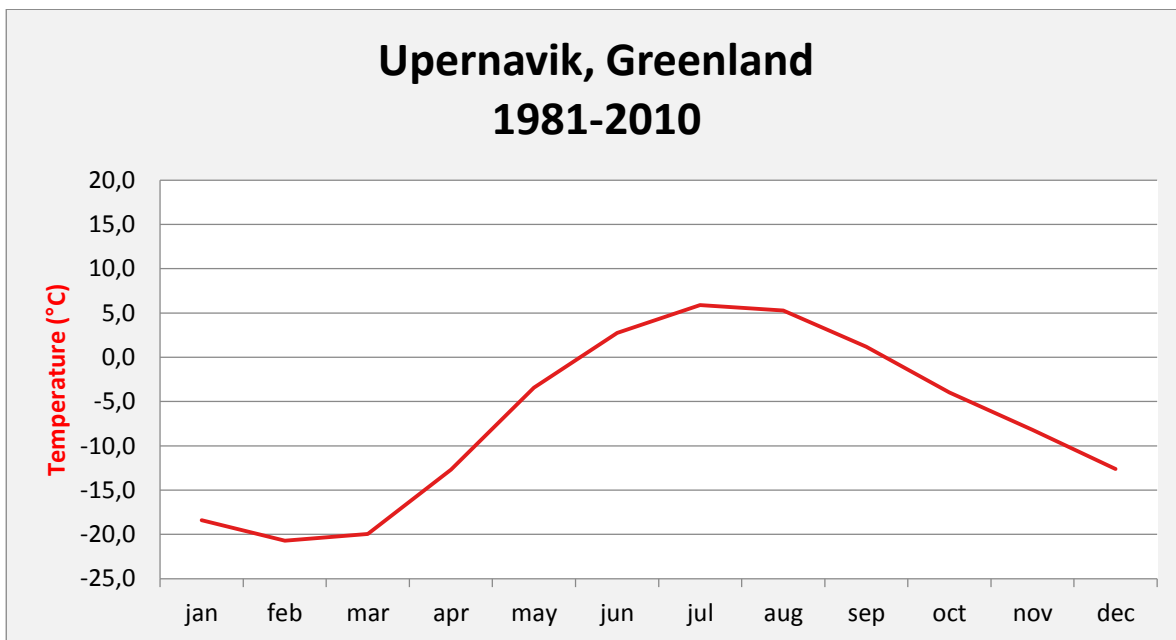
Figure 19. Average monthly values for the period 1981-2010; air temperature. 4211 Upernavik, Greenland.
