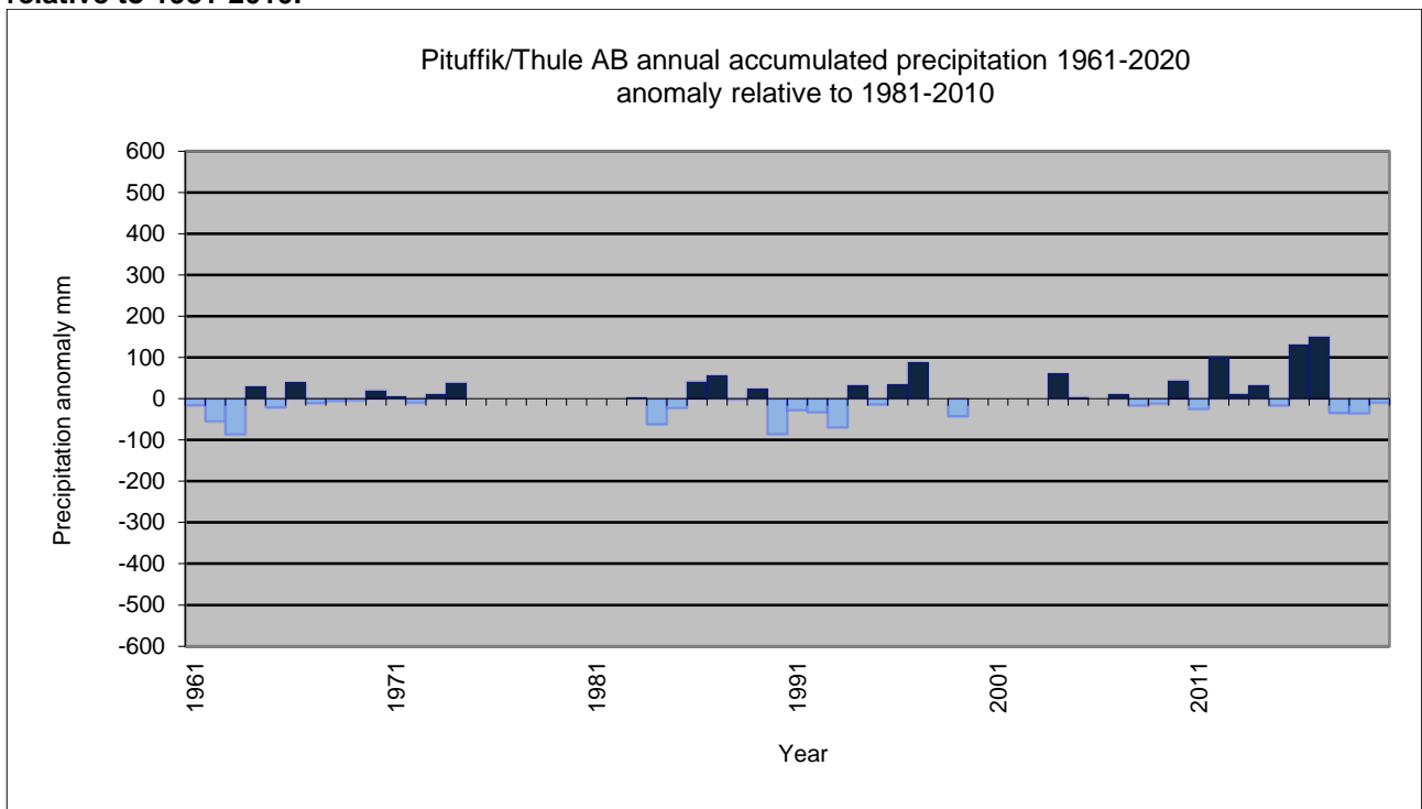
Figure 16. Annual accumulated precipitation since 1961. 4202 Pituffik/Thule AB, Greenland. Anomaly relative to 1981-2010.
