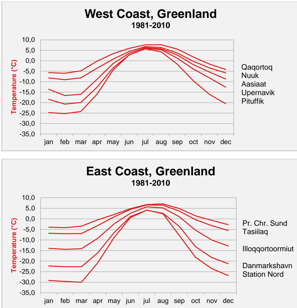
Figure 7. Monthly mean temperatures (average over period 1981-2010) for selected stations at the Greenland west coast (upper figure) and east coast (lower figure).
