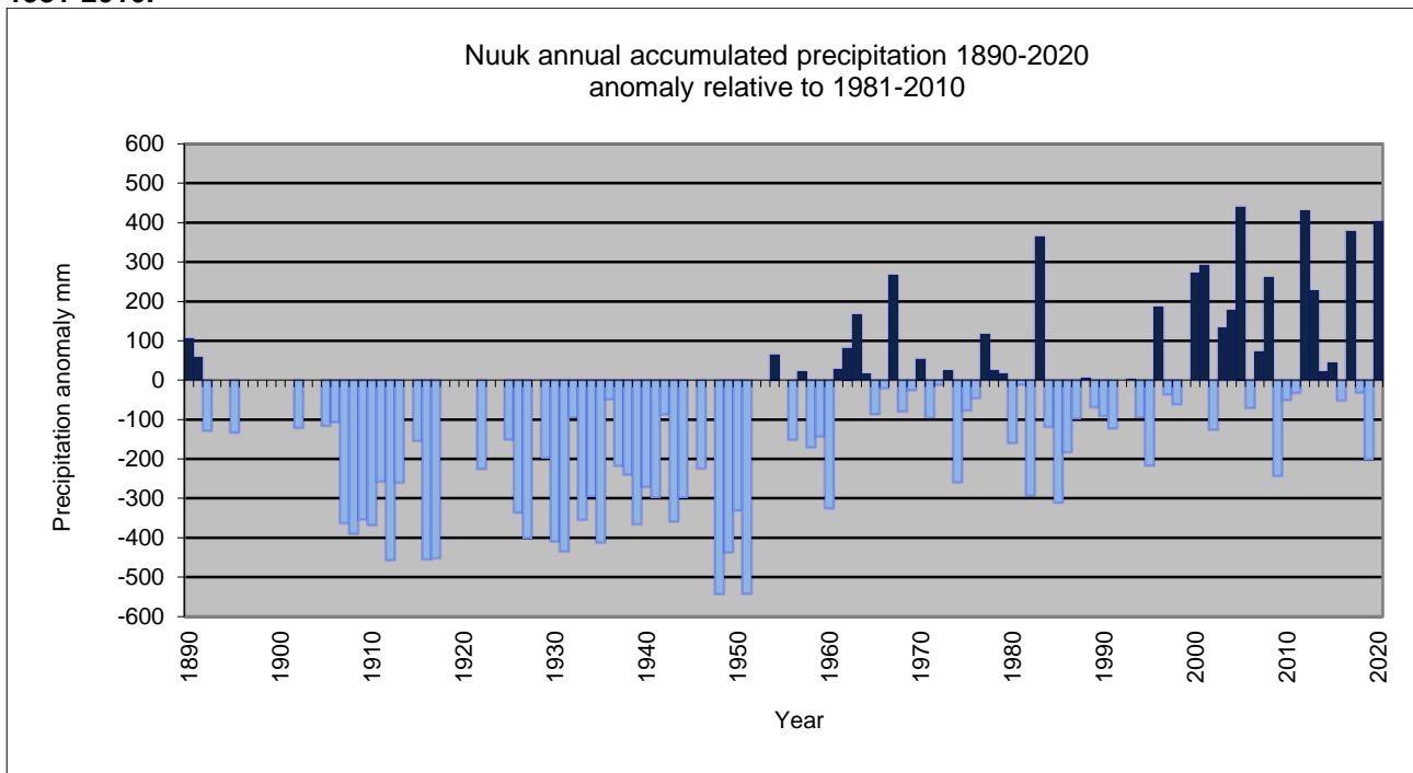
Figure 23. Annual accumulated precipitation since 1890; 4250 Nuuk, Greenland. Anomaly relative to 1981-2010.
