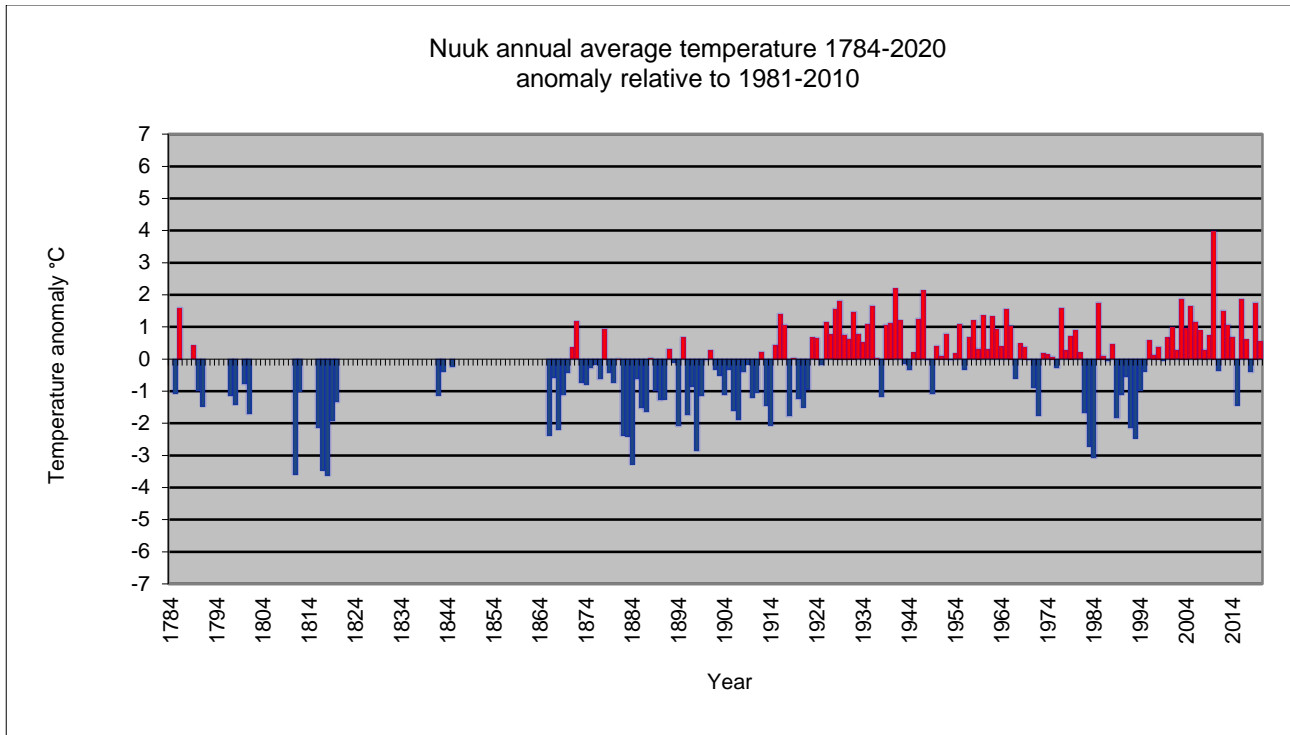
Figure 22. Annual average air temperature since 1784. 4250 Nuuk, Greenland. Anomaly relative to 1981-2010.
