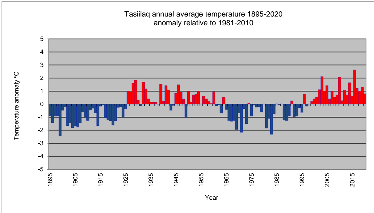
Figure 37. Annual average air temperature since 1895. 4360 Tasiilaq, Greenland. Anomaly relative to 1981-2010.
