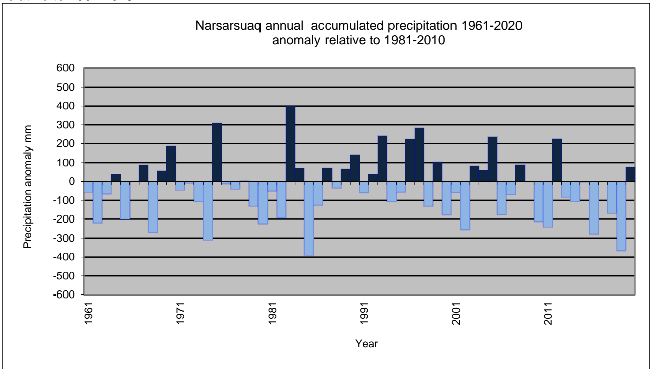
Figure 26. Annual accumulated precipitation since 1961; 4270 Narsarsuaq, Greenland. Anomaly relative to 1981-2010.
