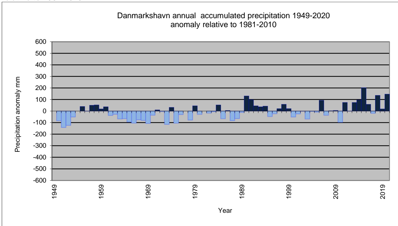
Figure 32. Annual accumulated precipitation since 1949; 4320 Danmarkshavn, Greenland. Anomaly relative to 1981-2010.
