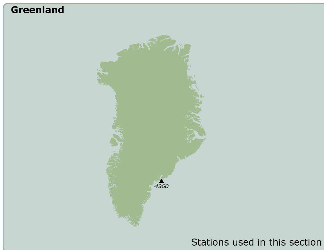
Figure 10. Map showing station position, 04360 Tasiilaq, Greenland.
