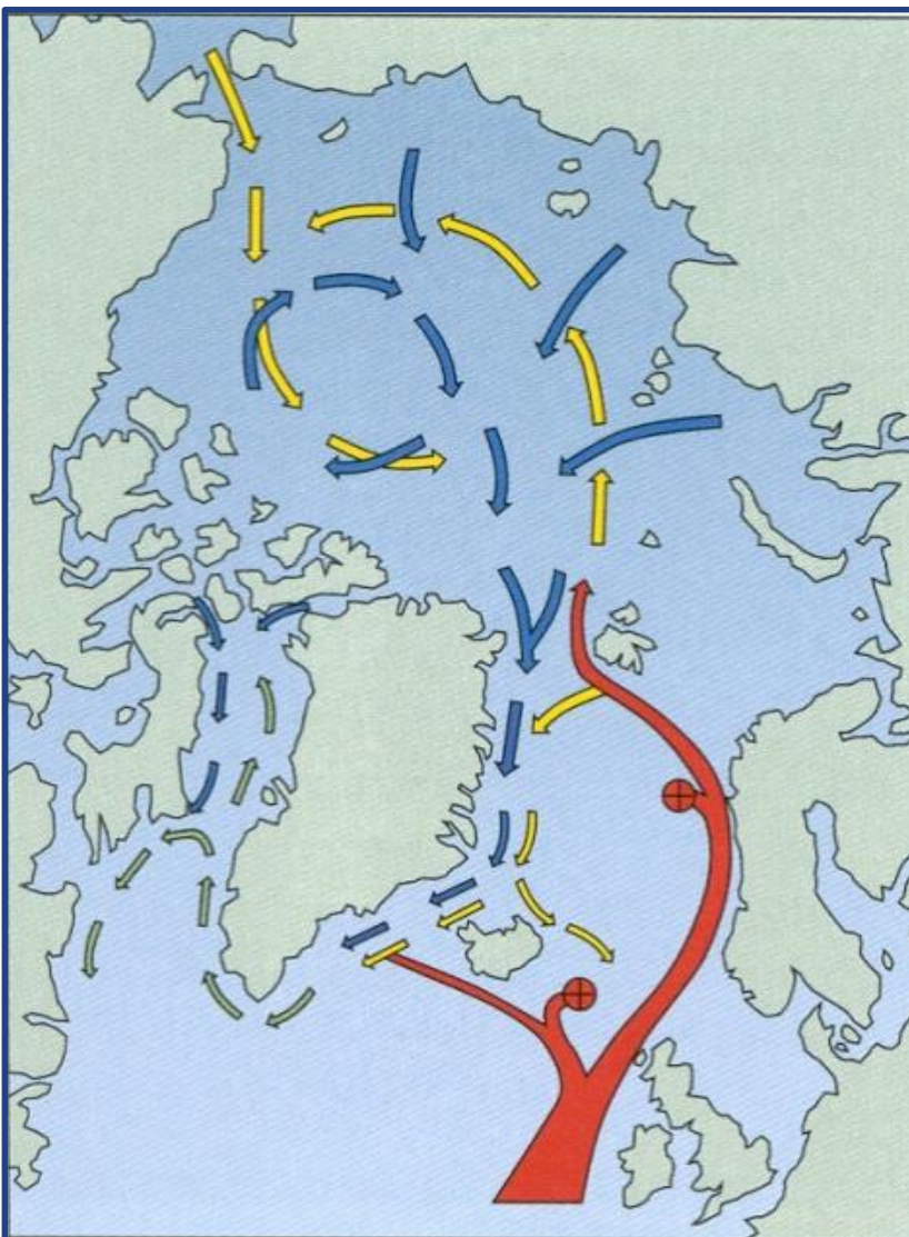
Figure 3. Sea currents in the Arctic Ocean and the North Atlantic Ocean.
