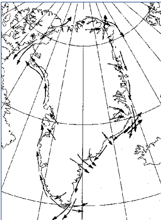
Figure 6. Predominant wind directions in situations with strong winds in the coastal area.
