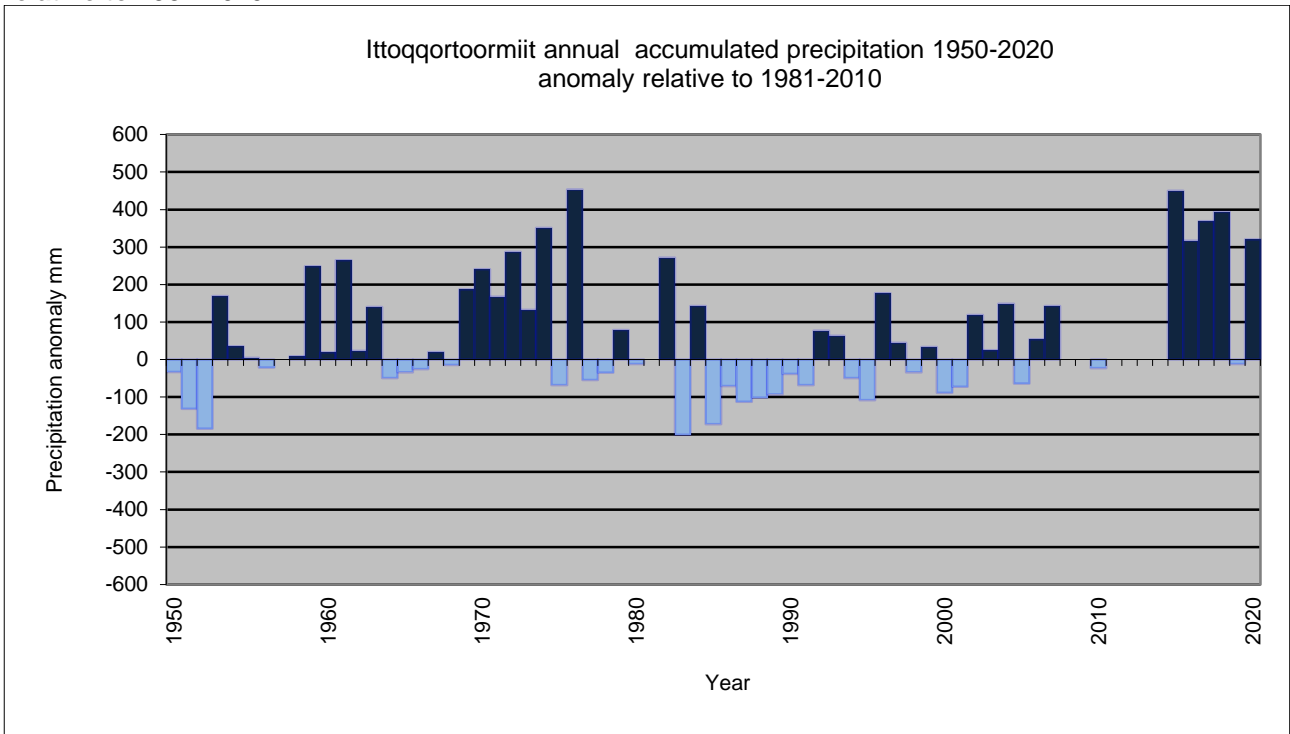
Figure 35. Annual accumulated precipitation since 1950; 4339 Ittoqqortoormiit, Greenland. Anomaly relative to 1981-2010.
