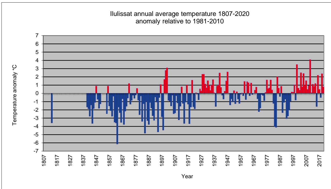
Figure 20. Annual average air temperature since 1807. 4221 Ilulissat, Greenland. Anomaly relative to 1981-2010.
