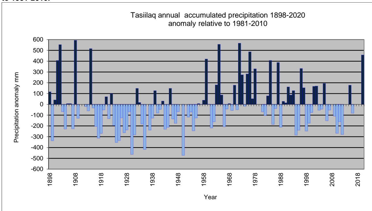
Figure 38. Annual accumulated precipitation since 1898; 4360 Tasiilaq, Greenland. Anomaly relative to 1981-2010.
