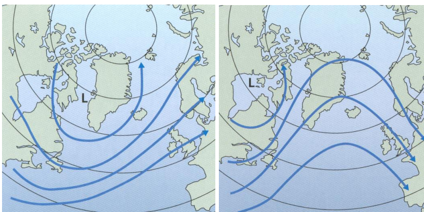
Figure 8. “The Temperature Seesaw” - sketch illustration of the two deviating 500 hPa patterns in NAO (North Atlantic Oscillation). Source: Leif Rasmussen.
