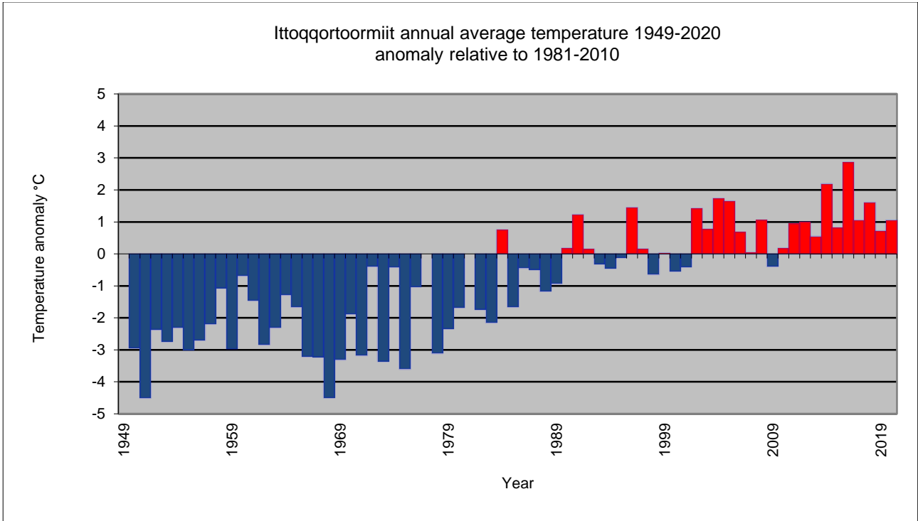
Figure 34. Annual average air temperature since 1949. 4339 Ittoqqortoormiit, Greenland. Anomaly relative to 1981-2010.
