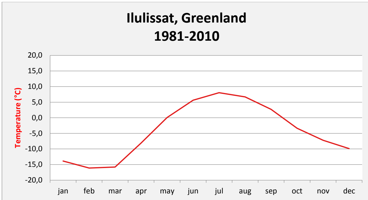
Figure 21. Average monthly values for the period 1981-2010; air temperature. 4221 Ilulissat, Greenland.
