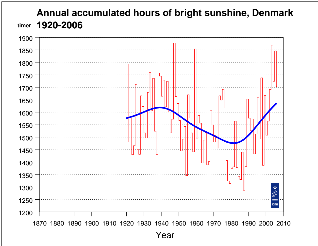
Figure 6. Annual accumulated hours of bright sunshine, Denmark 1920-2006. A Gauss filter with filter width (standard deviation) 9 years has been used to create the “bold” smooth curve. A Gauss filter with standard deviation 9 years is comparable to a 30-years running mean. However, the filter gives a smoother curve than a running mean, as sunshine values from central years are given larger weight than sunshine values from periferal years. Filter values are also calculated for the years at either end of the series. It should be noted that these values are computed from one-sided Gauss filters, and that values from later years will change when the series is updated.
