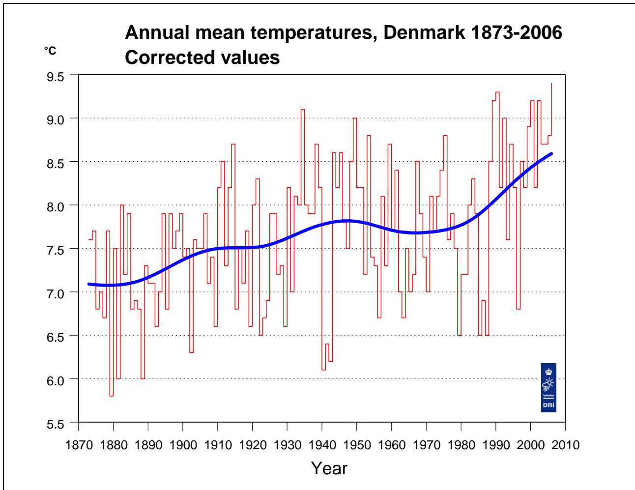
Figure 4. Annual mean temperature, Denmark 1873-2006, corrected values. A Gauss filter with filter width (standard deviation) 9 years has been used to create the “bold” smooth curve. A Gauss filter with standard deviation 9 years is comparable to a 30-years running mean. However, the filter gives a smoother curve than a running mean, as temperature values from central years are given larger weight than temperature values from periferal years. Filter values are also calculated for the years at either end of the series. It should be noted that these values are computed from one-sided Gauss filters, and that values from later years will change when the series is updated.
