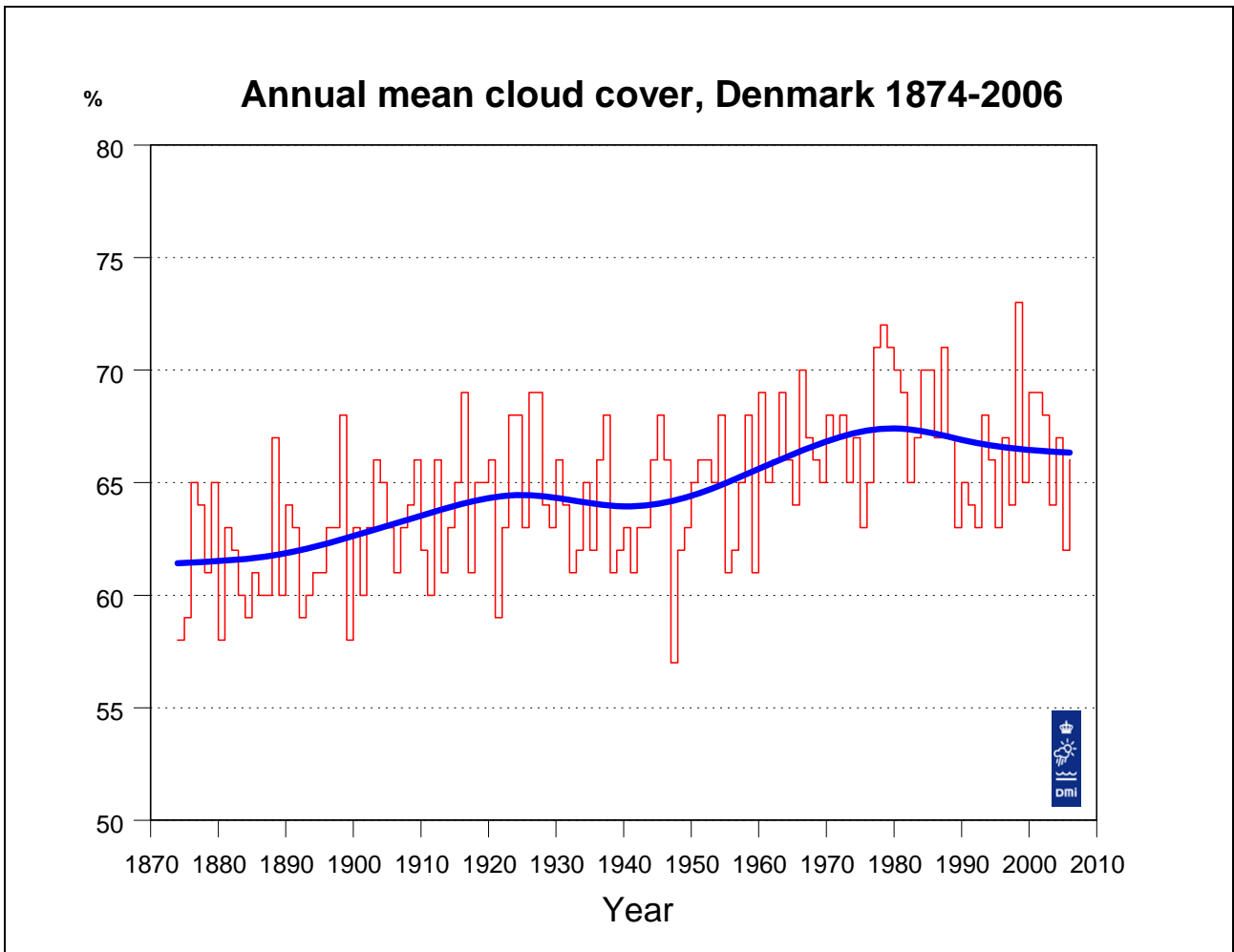
Figure 7. Annual mean cloud cover, Denmark 1874-2006. A Gauss filter with filter width (standard deviation) 9 years has been used to create the “bold” smooth curve. A Gauss filter with standard deviation 9 years is comparable to a 30-years running mean. However, the filter gives a smoother curve than a running mean, as cloud cover values from central years are given larger weight than cloud cover values from periferal years. Filter values are also calculated for the years at either end of the series. It should be noted that these values are computed from one-sided Gauss filters, and that values from later years will change when the series is updated.
