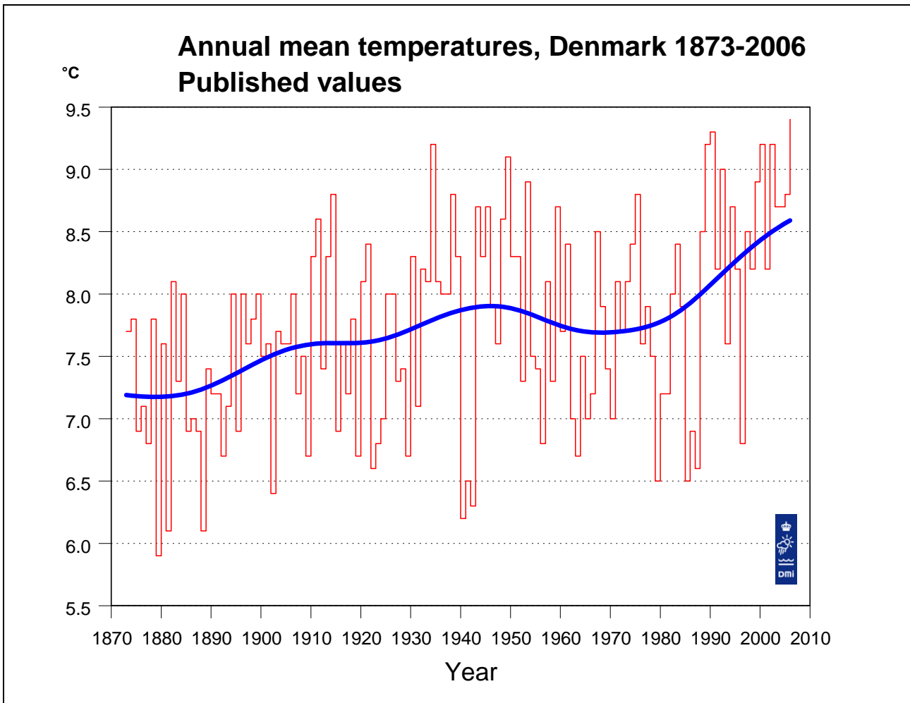
Figure 3. Annual mean temperature, Denmark 1873-2006, published values. A Gauss filter with filter width (standard deviation) 9 years has been used to create the “bold” smooth curve. A Gauss filter with standard deviation 9 years is comparable to a 30-years running mean. However, the filter gives a smoother curve than a running mean, as temperature values from central years are given larger weight than temperature values from periferal years. Filter values are also calculated for the years at either end of the series. It should be noted that these values are computed from one-sided Gauss filters, and that values from later years will change when the series is updated.
