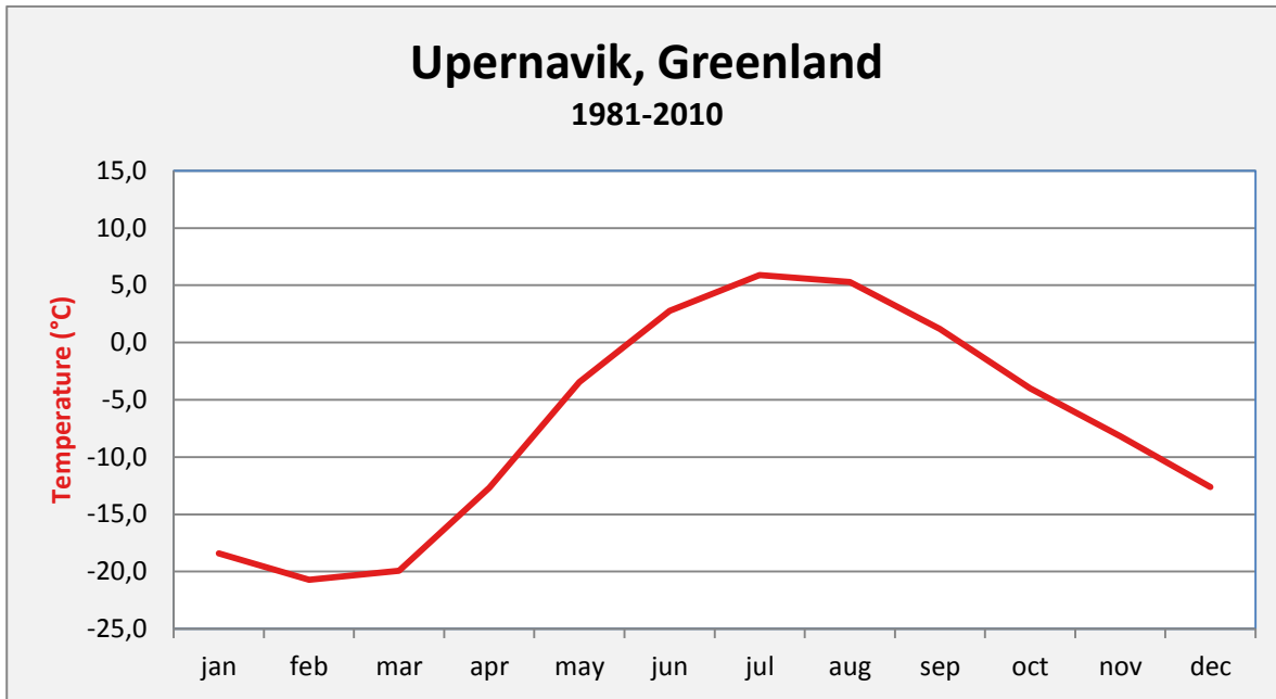
Annual average air temperature for 4211 Upernavik 1981-2010. Observations of precipitation stopped in 1981.
