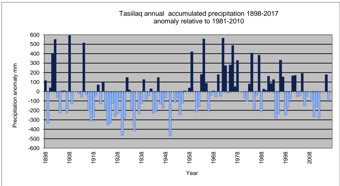
Annual accumulated precipitation since 1898 for 4360 Tasillaq; anomaly relative to 1981-2010. There are missing values for some years 1910-1911, 1936, 1949, 1951, 1979-1980, 2008 and 2013-2014.
