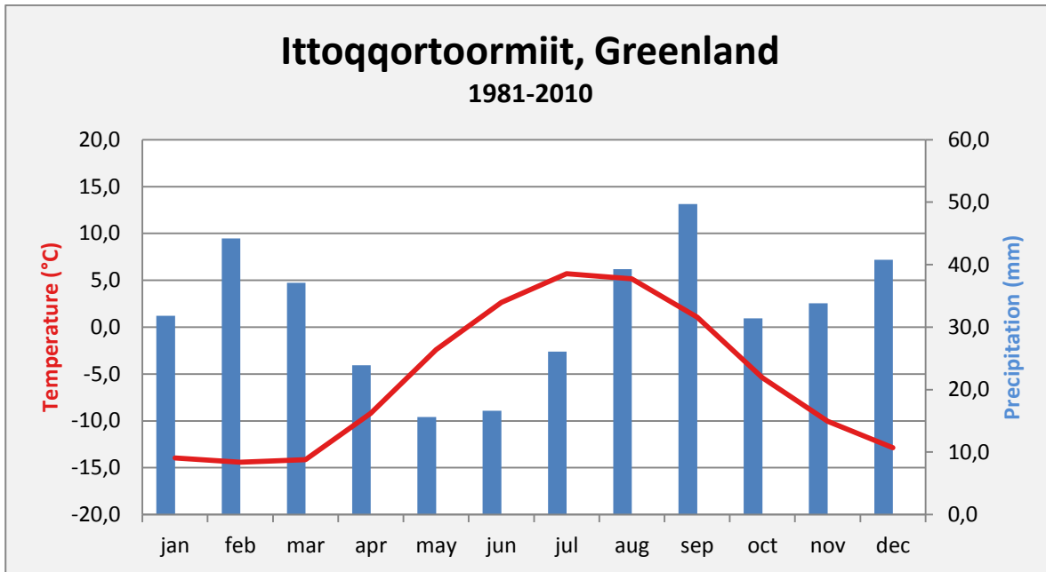
Annual average air temperature and annual accumulated precipitation for 4339 Ittoqqortoormiit 1981-2010.
