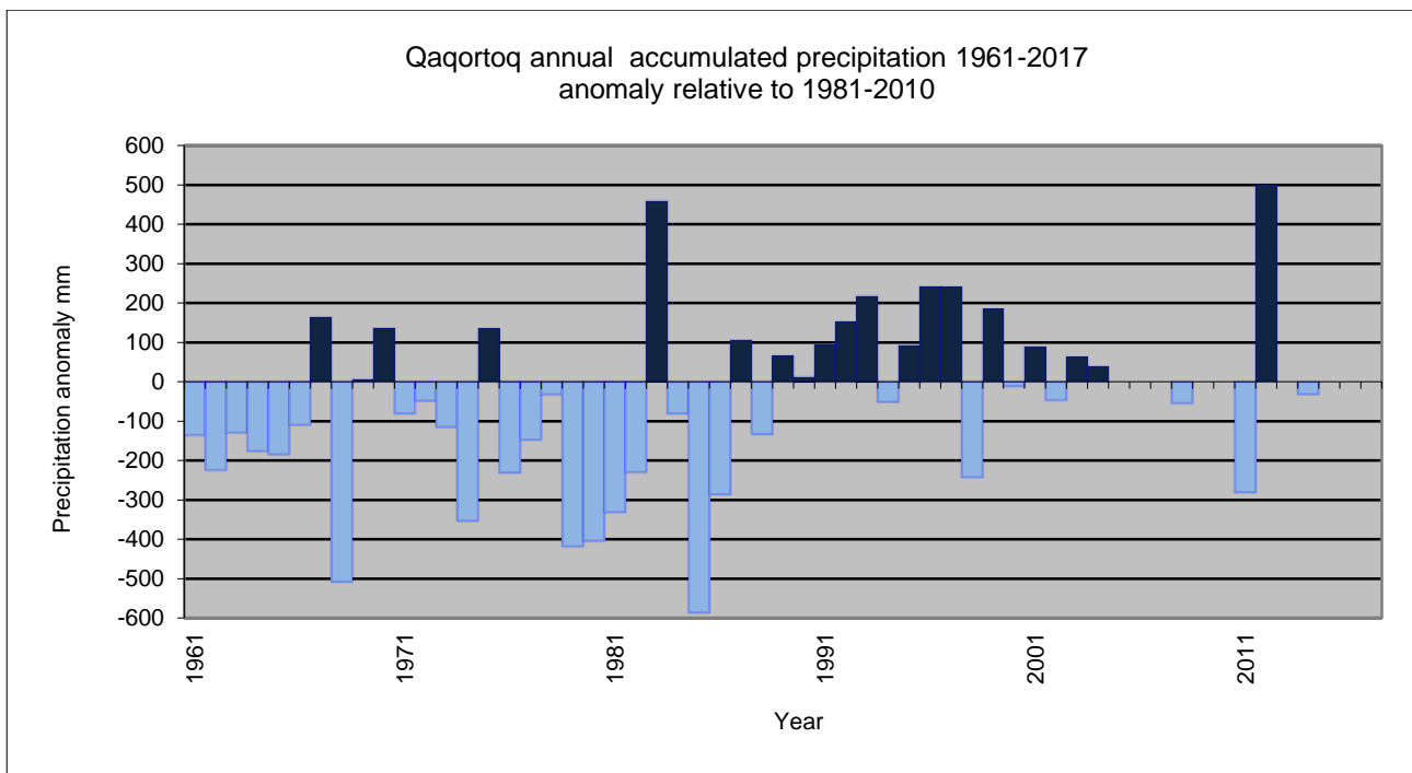
Annual accumulated precipitation since 1961 for 4272 Qaqortoq; anomaly relative to 1981-2010. There are missing values for some years 2005-2007, 2009-2010, 2013 and 2015-2017.
