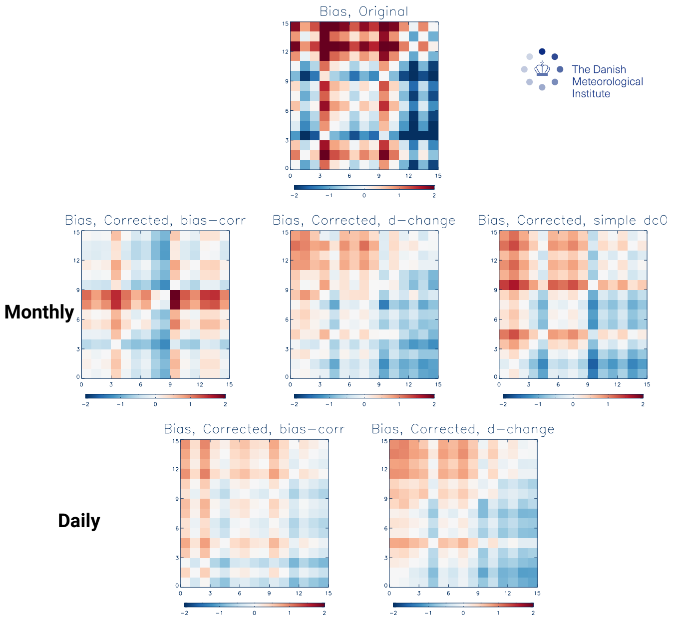
Figure 6: The difference between mean climates in calibrated models and ‘truth’. January near-surface temperature. Calibration period 1971-2000, prediction period: 2070-2099. Scenario: RCP8.5. The numbers on the axes refer to the model combinations in Table 2. The horizontal axes indicates the model selected as ‘truth’. Top panel shows uncalibrated values. In middle panes calibration is performed on monthly means, in lower panels on daily means.
