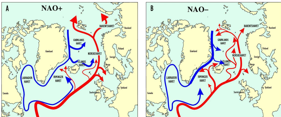
Figure 9. Schematic surface circulation during a) high NAO index, and b) low NAO index. From Blindheim et al. (2001).
