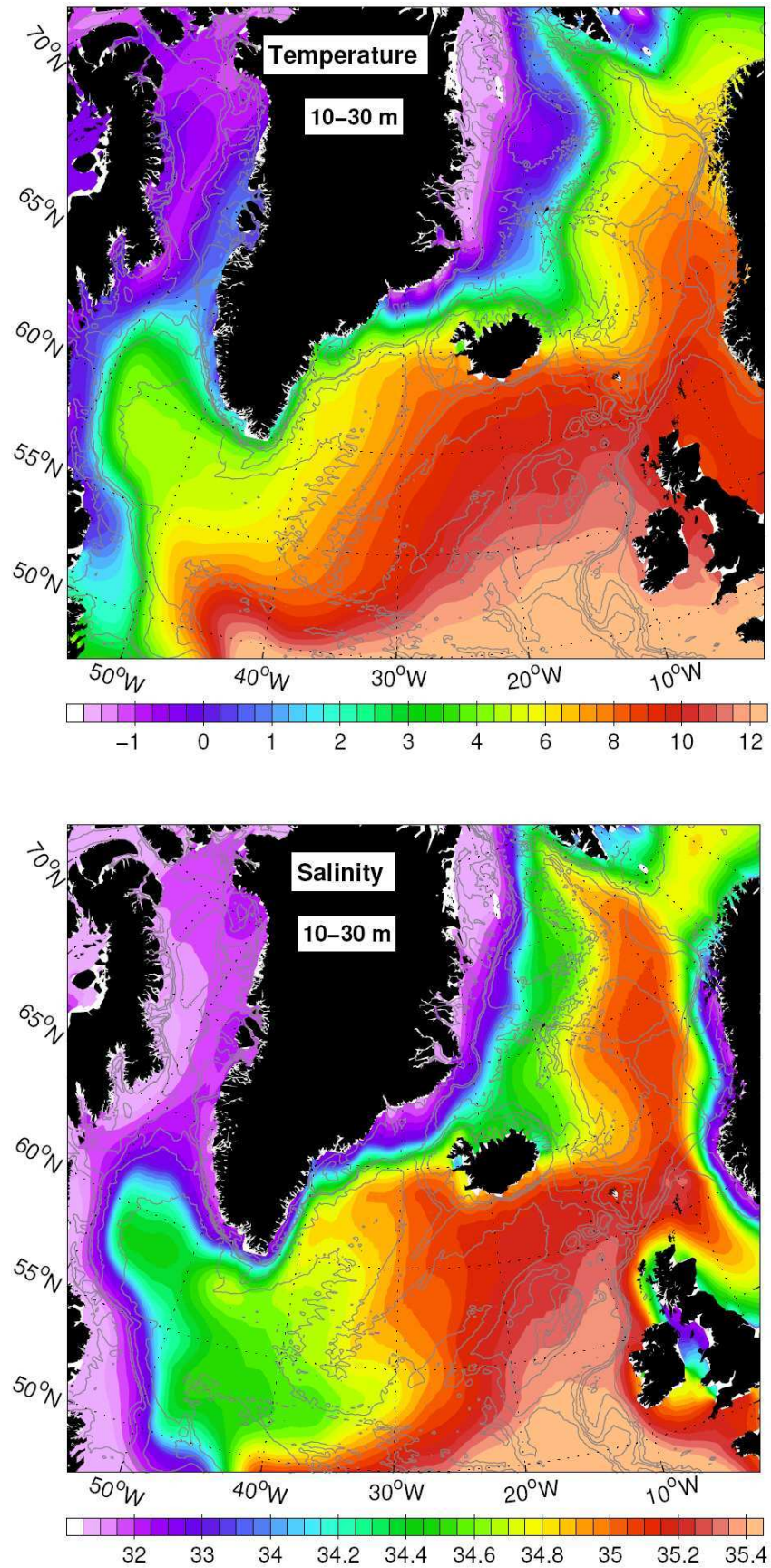
Figure 6. Annual mean surface (10–30 m) temperature (top) and salinity (bottom) from World Ocean Atlas 2001 (WOA2001). Note the change in scales at 4°C for temperature and 34 for salinity. Bottom contours at 500, 1000, 2000, 3000 and 4000 m are shown.
