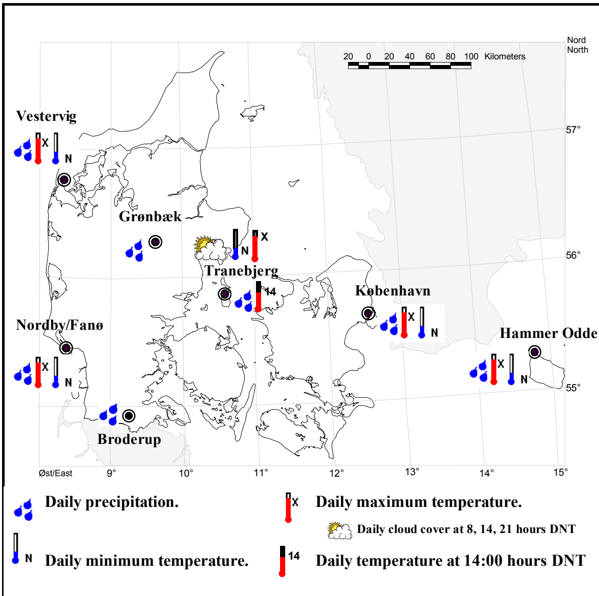
Figure 2.1. The seven Danish sites with digitised daily precipitation, temperature and/or cloud cover observations, 1874-2006. The stations representing each site are listed in the tables 3.1 – 3.5. For station co-ordinates confer with the station position file in the data files included. DNT refers to Danish normal time, which is the time in a given time zone in contrast to summer time, where 1 hour is added. In Denmark the normal time is UTC+1.
