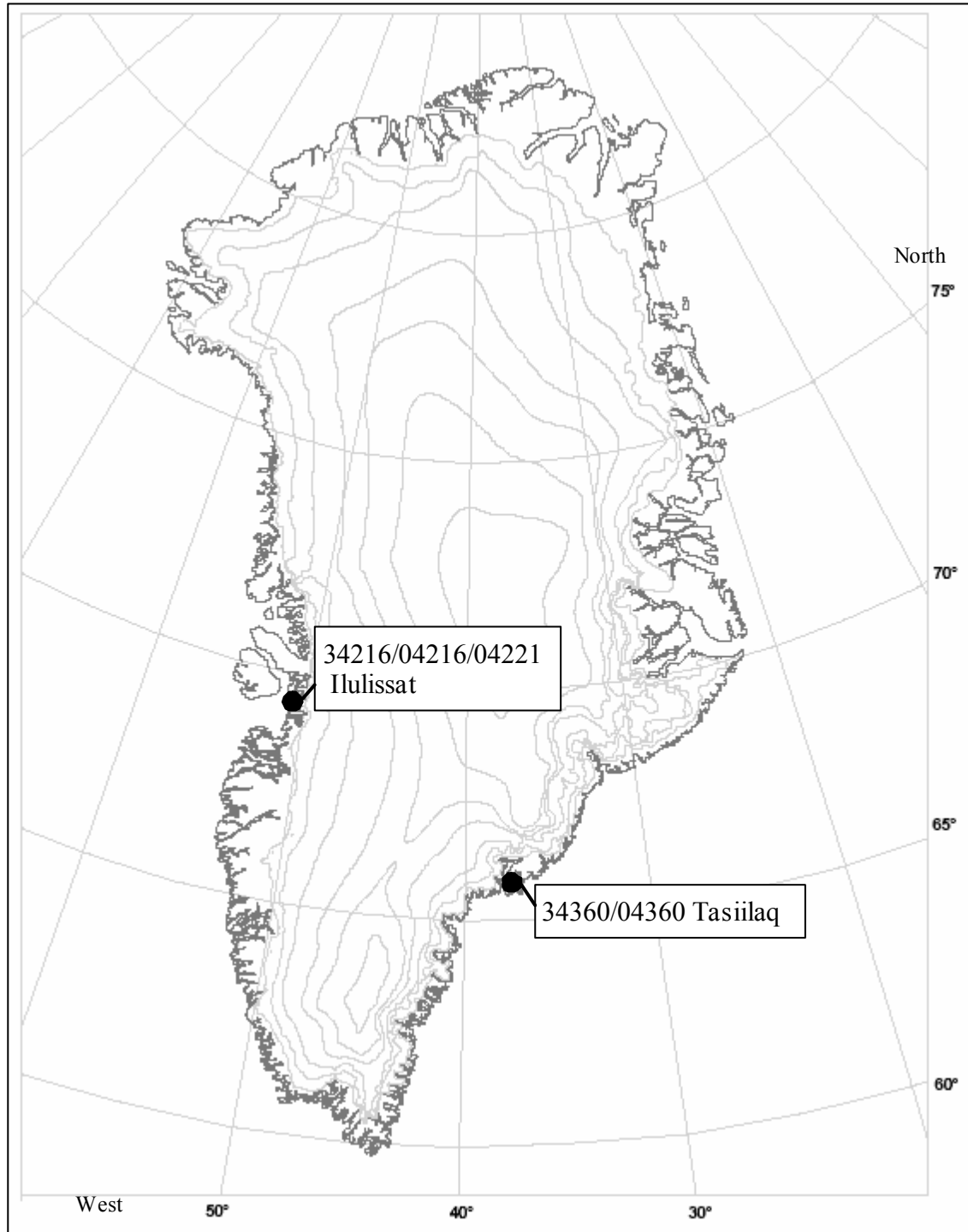
Figure 2.3. The location of the two Greenlandic sites with long daily data series: Ilulissat (formerly: Jacobshavn) on the West Coast and Tasiilaq (formerly: Angmagssalik) on the East Coast, 1873-2006. The stations representing each site are listed in the tables 4.1 – 4.3. For station co-ordinates confer with the station position file in the data files included.
