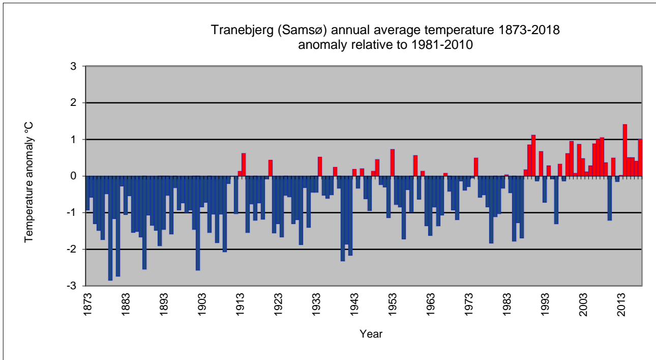
Figure 8.2.9. Annual average air temperature, Tranebjerg (Samsø), 1873-2018, anomaly relative to 1981-2010.
