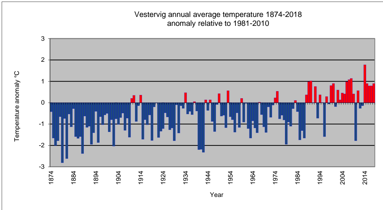
Figure 8.2.5. Annual average air temperature, Vestervig 1874-2018, anomaly relative to 1981-2010.
