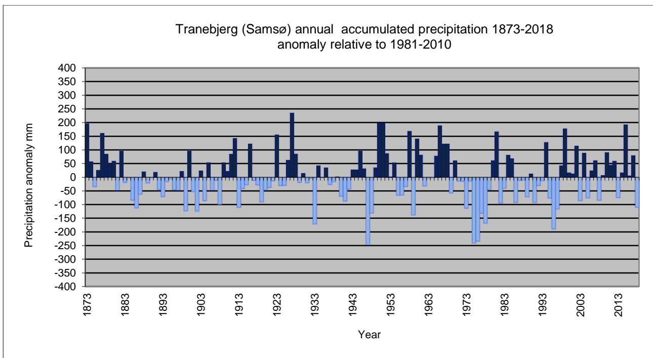
Figure 8.2.10. Annual accumulated precipitation, Tranebjerg (Samsø), 1873-2018, anomaly relative to 1981-2010.
