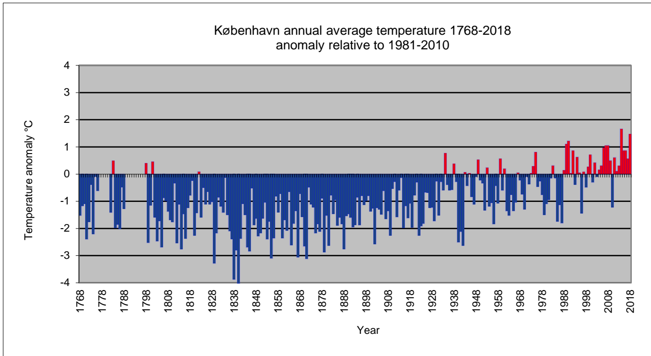
Figure 8.2.11. Annual average air temperature, København, 1768-2018, anomaly relative to 1981-2010. There are missing values for some early years 1777-1781 and 1789-1797.
