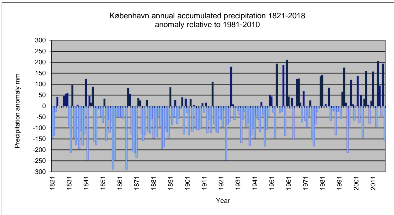
Figure 8.2.12. Annual accumulated precipitation, København, 1821-2018, anomaly relative to 1981-2010. There are missing values for some early years 1825-1826.
