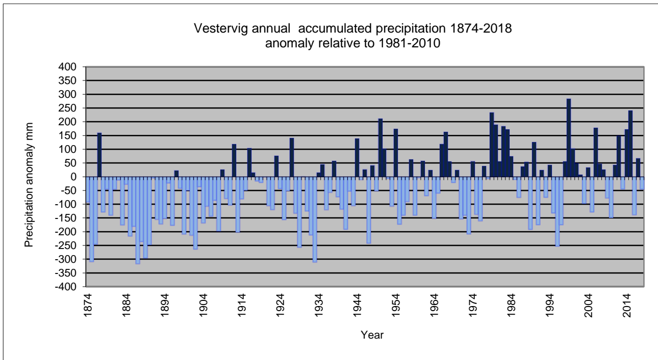
Figure 8.2.6. Annual accumulated precipitation, Vestervig 1874-2018, anomaly relative to 1981-2010.
