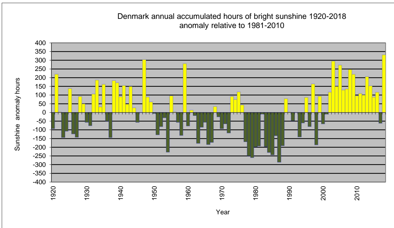
Figure 8.2.4. Annual accumulated hours of bright sunshine, Denmark 1920-2018, anomaly relative to 1981-2010. OBS! DMI has since 2002 observed the hours of bright sunshine using measurements of global radiation instead of measurements from a traditional Campbell-Stokes sunshine recorder. For that reason “new” and “old” hours of bright sunshine cannot directly be compared. It should be noted that all values before 2002 are adjusted ensuring comparability to the new level. For details on that, see [33].
