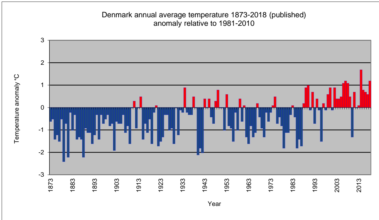
Figure 8.2.1. Annual average air temperature (published values), Denmark 1873-2018, anomaly relative to 1981-2010.
