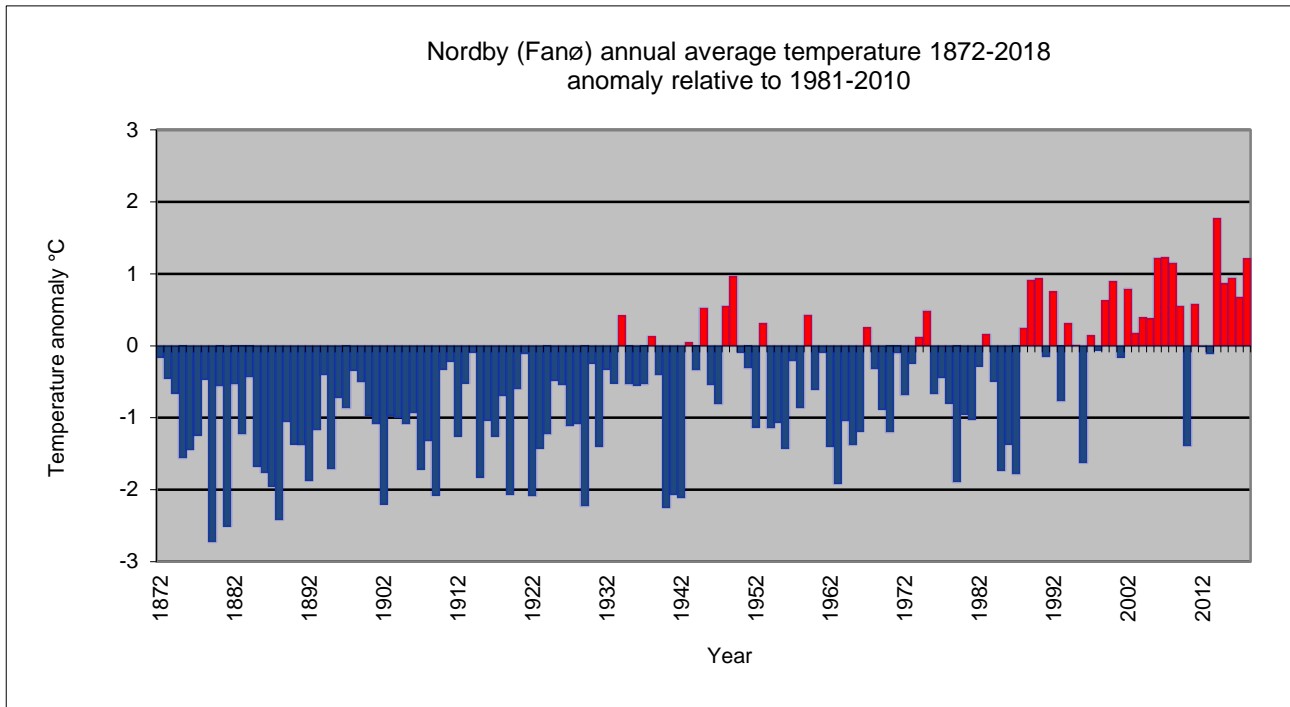
Figure 8.2.7. Annual average air temperature, Nordby (Fanø), 1872-2018, anomaly relative to 1981-2010.
