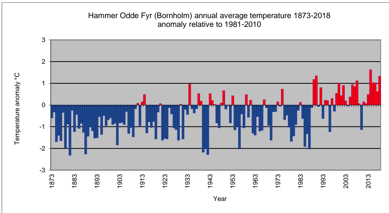
Figure 8.2.14. Annual average air temperature, Hammer Odde Fyr (Bornholm), 1873-2018, anomaly relative to 1981-2010.
