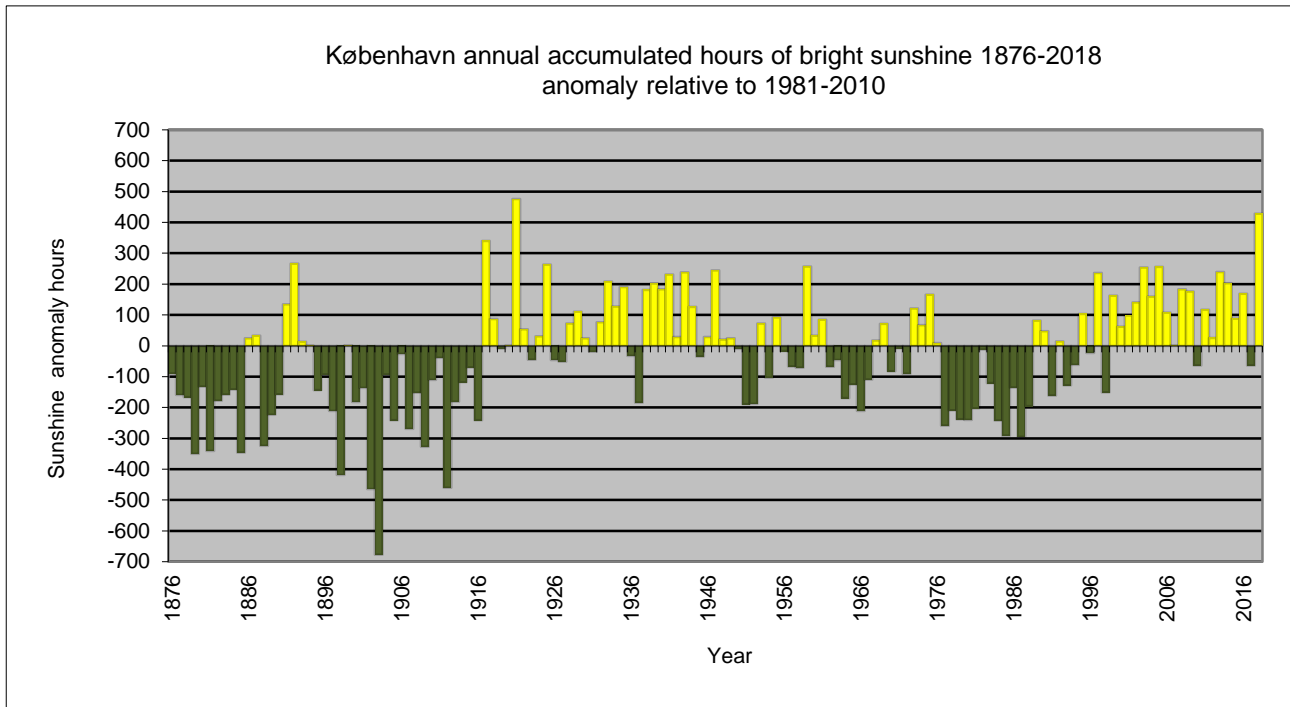
Figure 8.2.13. Annual accumulated hours of bright sunshine, København, 1876-2018, anomaly relative to 1981-2010. OBS! DMI has since 2002 observed the hours of bright sunshine using measurements of global radiation instead of measurements from a traditional Campbell-Stokes sunshine recorder. For that reason “new” and “old” hours of bright sunshine cannot directly be compared. It should be noted that all values before 2002 are adjusted ensuring comparability to the new level. For details on that, see [33].
