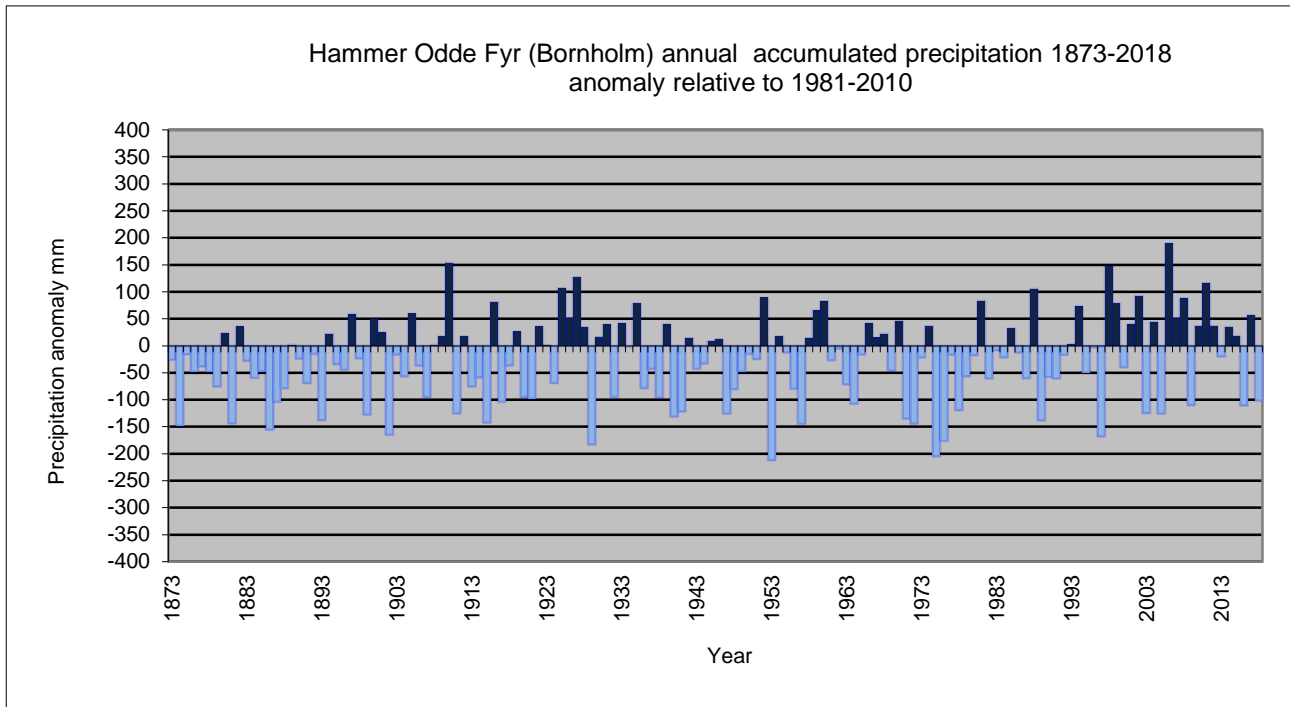
Figure 8.2.15. Annual accumulated precipitation, Hammer Odde Fyr (Bornholm), 1873-2018, anomaly relative to 1981-2010.
