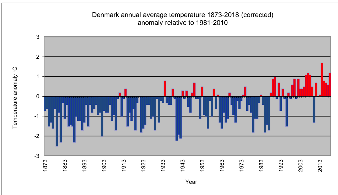
Figure 8.2.2. Annual average air temperature (corrected values), Denmark 1873-2018, anomaly relative to 1981-2010.
