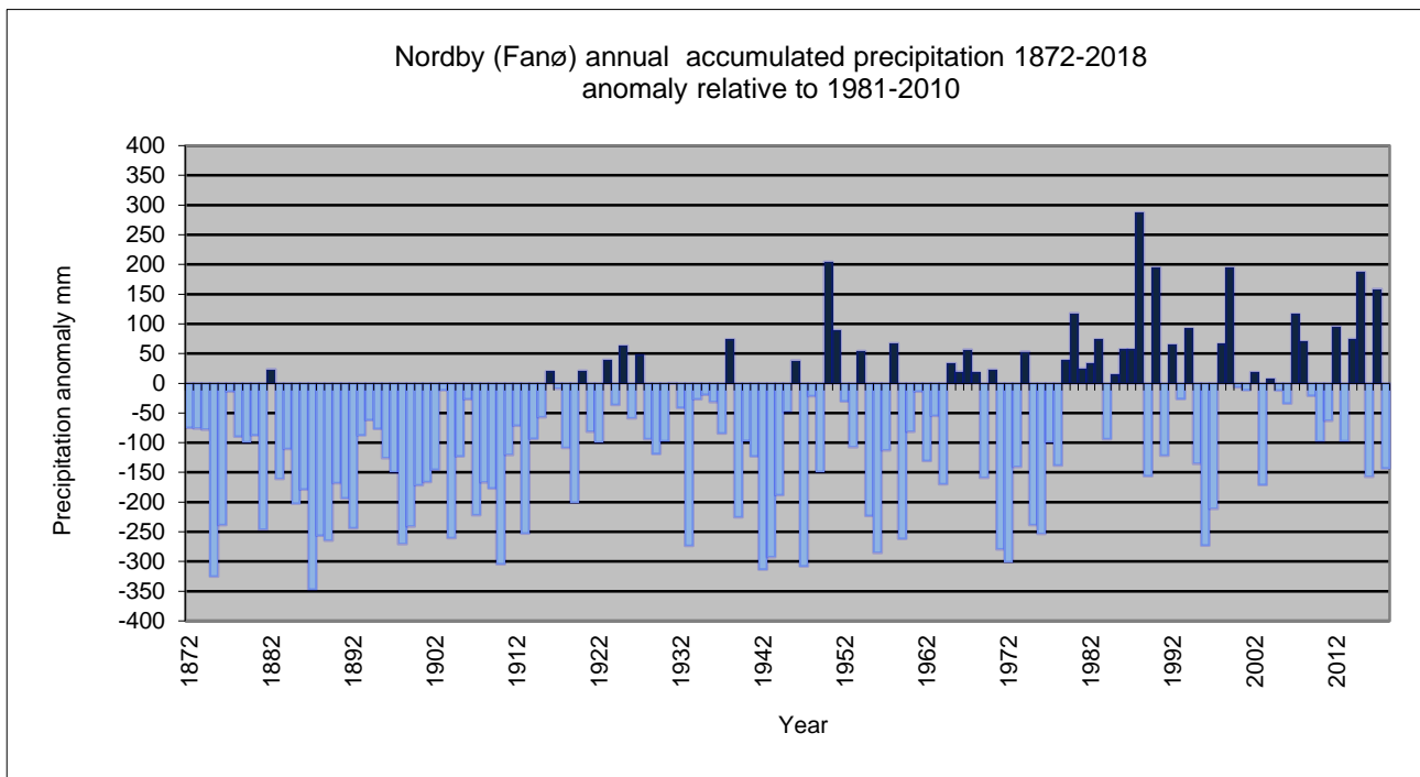
Figure 8.2.8. Annual accumulated precipitation, Nordby (Fanø), 1872-2018, anomaly relative to 1981-2010.
