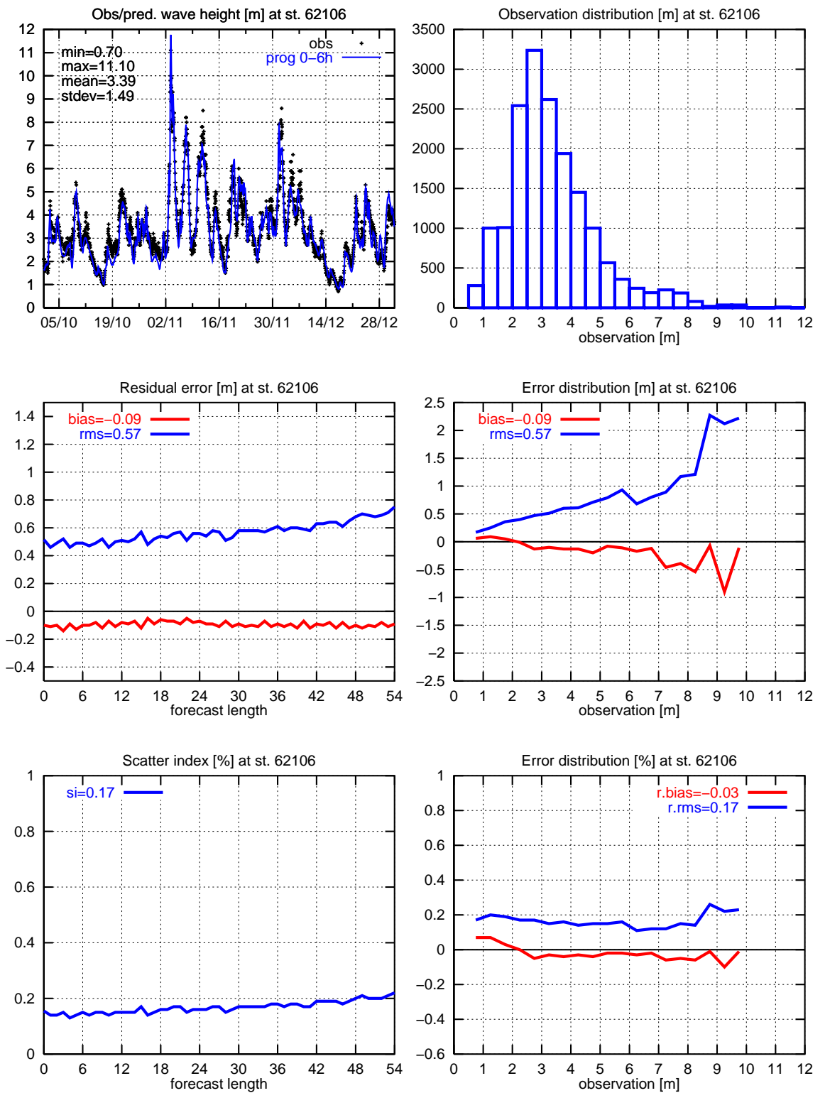
Figure 29. Significant wave height: 62106.
