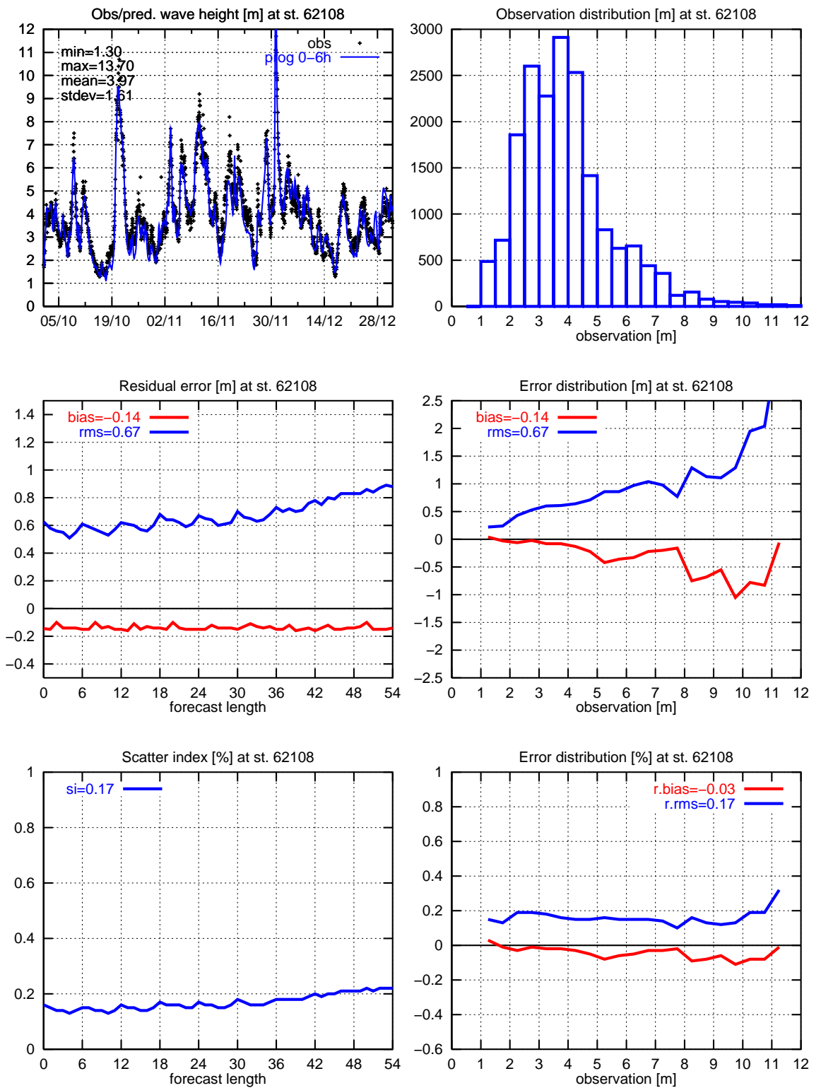
Figure 31. Significant wave height: 62108
