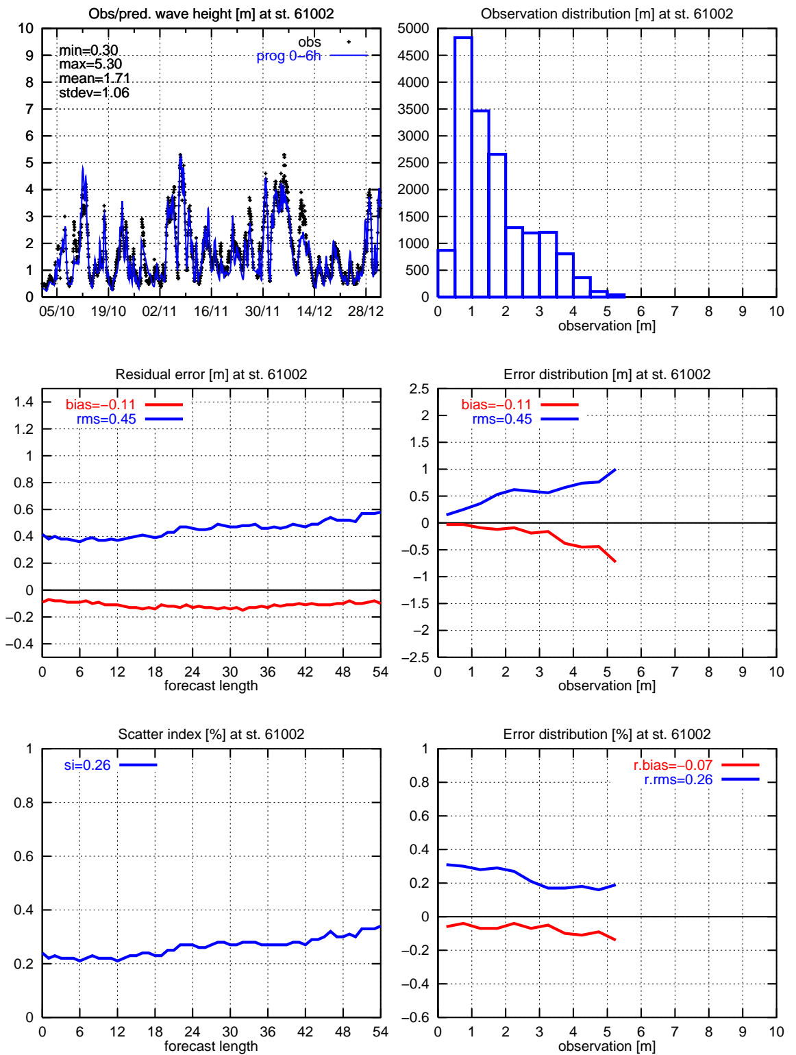
Figure 22. Significant wave height: 61002
