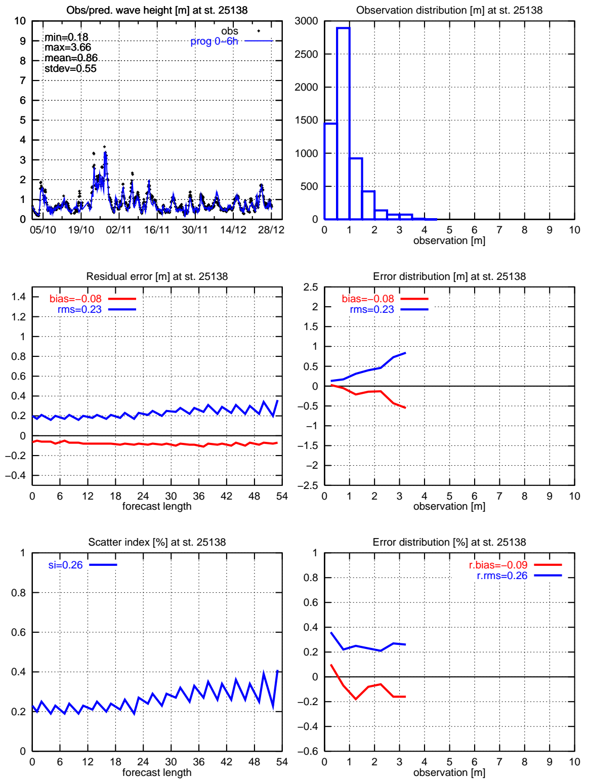
Figure 20. Significant wave height: 25138. The zig-zag curves are caused by irregular 3h sampling.
