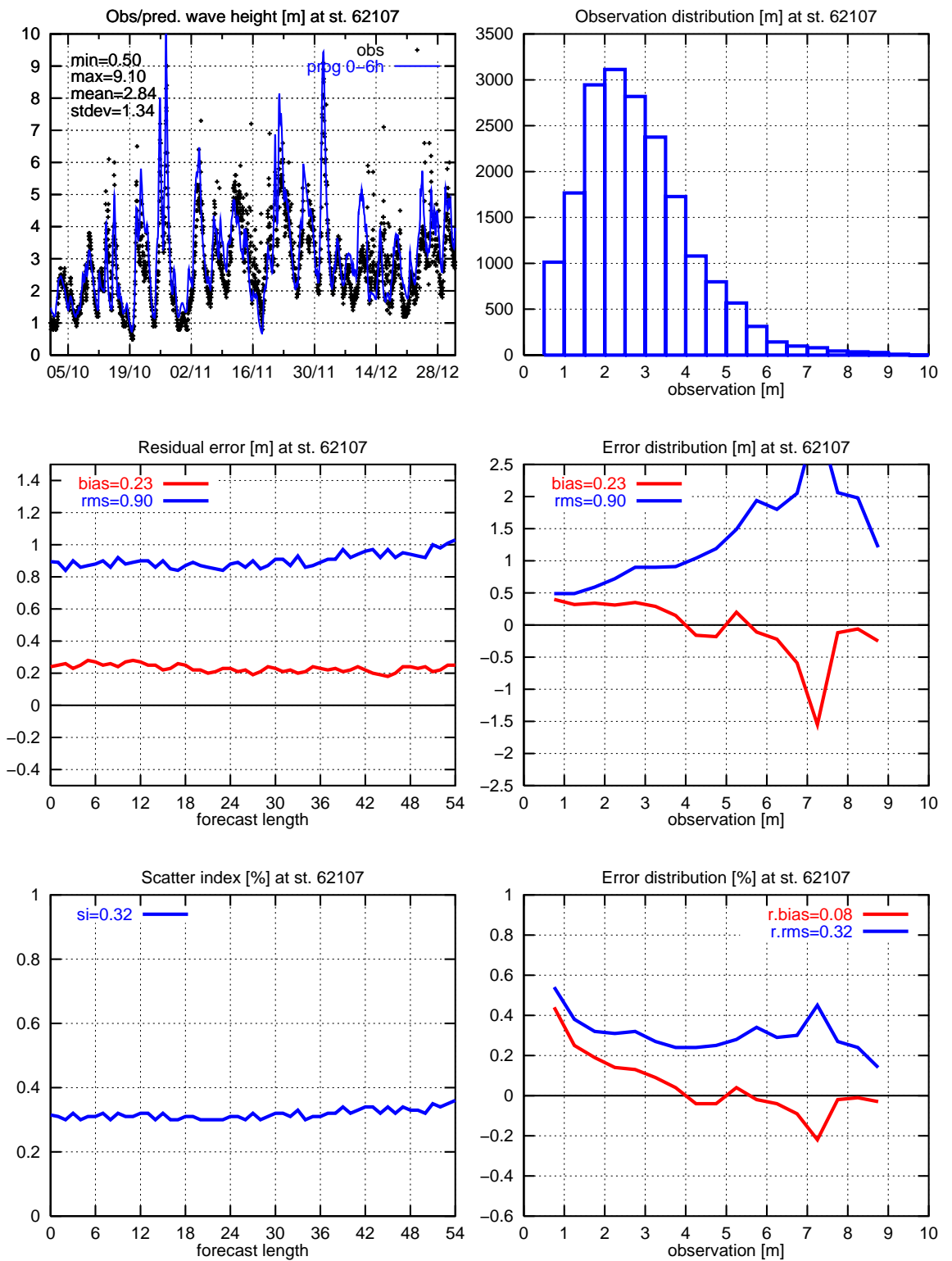
Figure 30. Significant wave height: 62107
