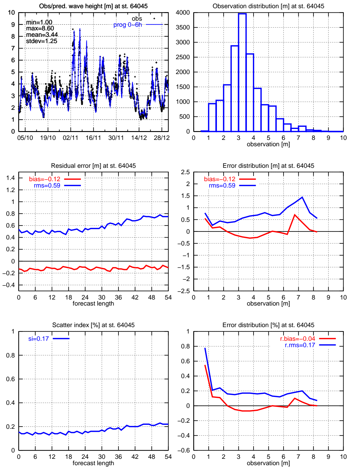
Figure 40. Significant wave height: 64045.
