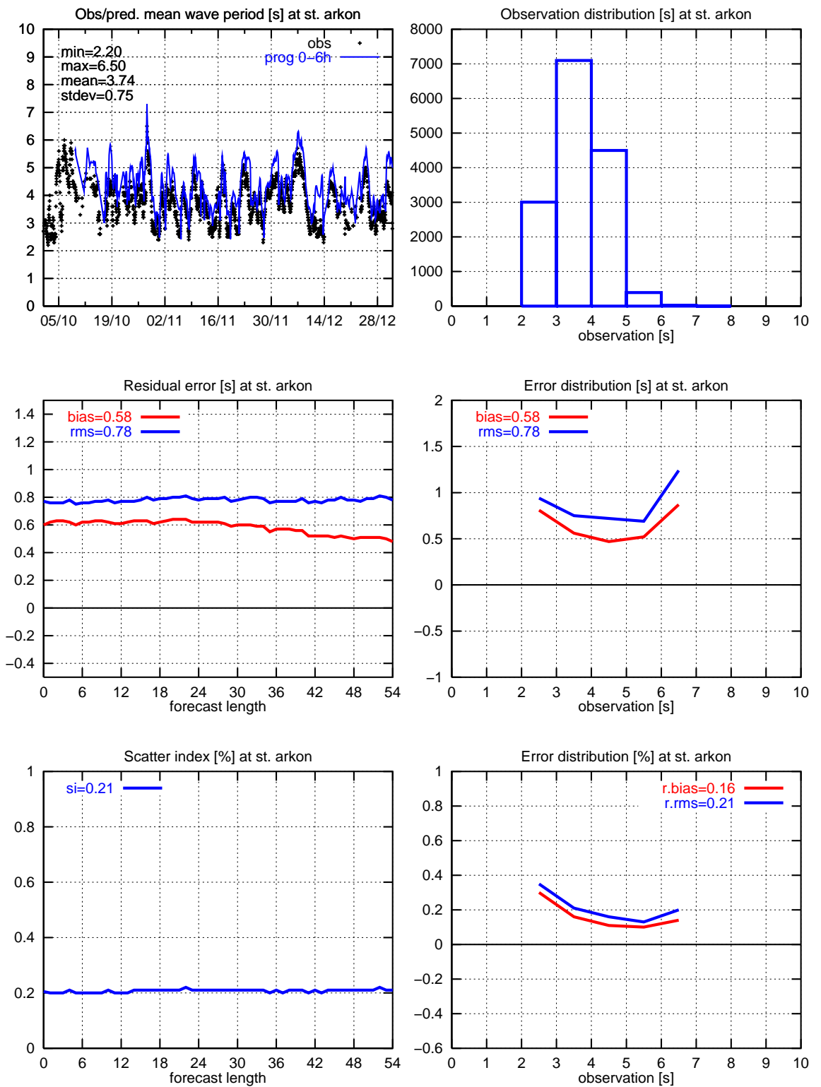
Figure 45. Mean wave period: Arkona
