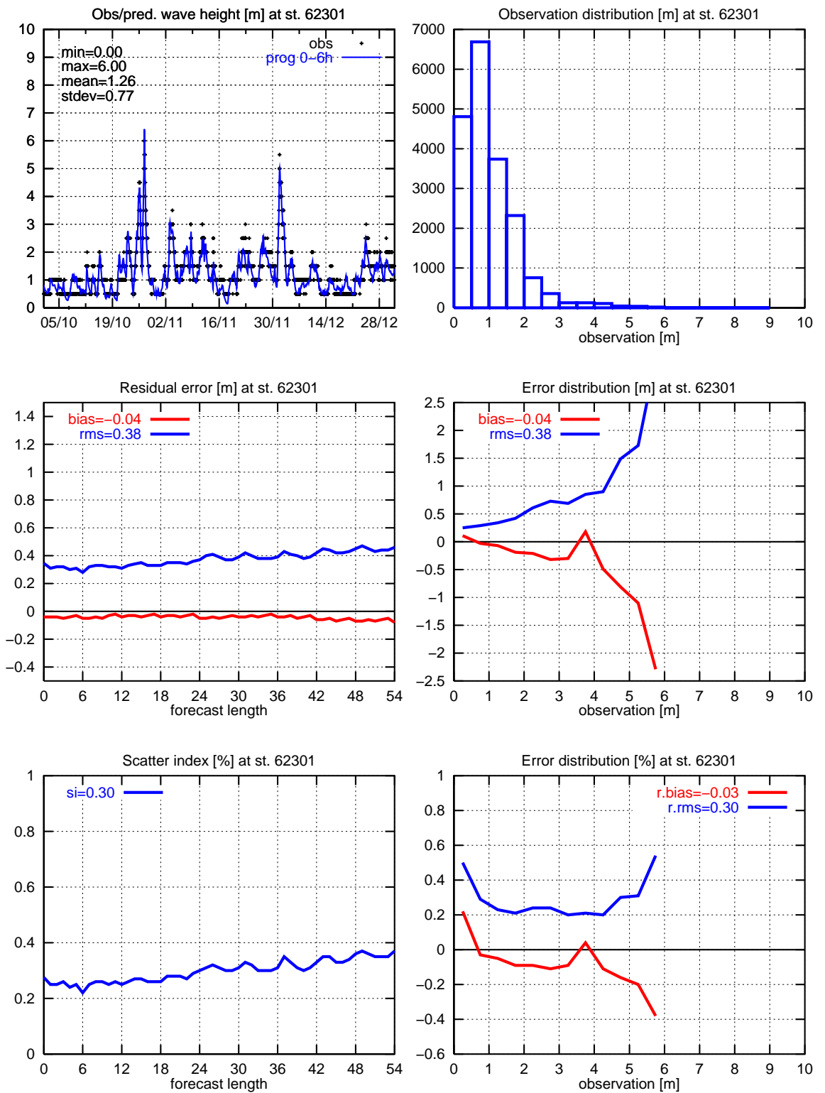
Figure 35. Significant wave height: 62301. The sampling accuracy is 0.5m
