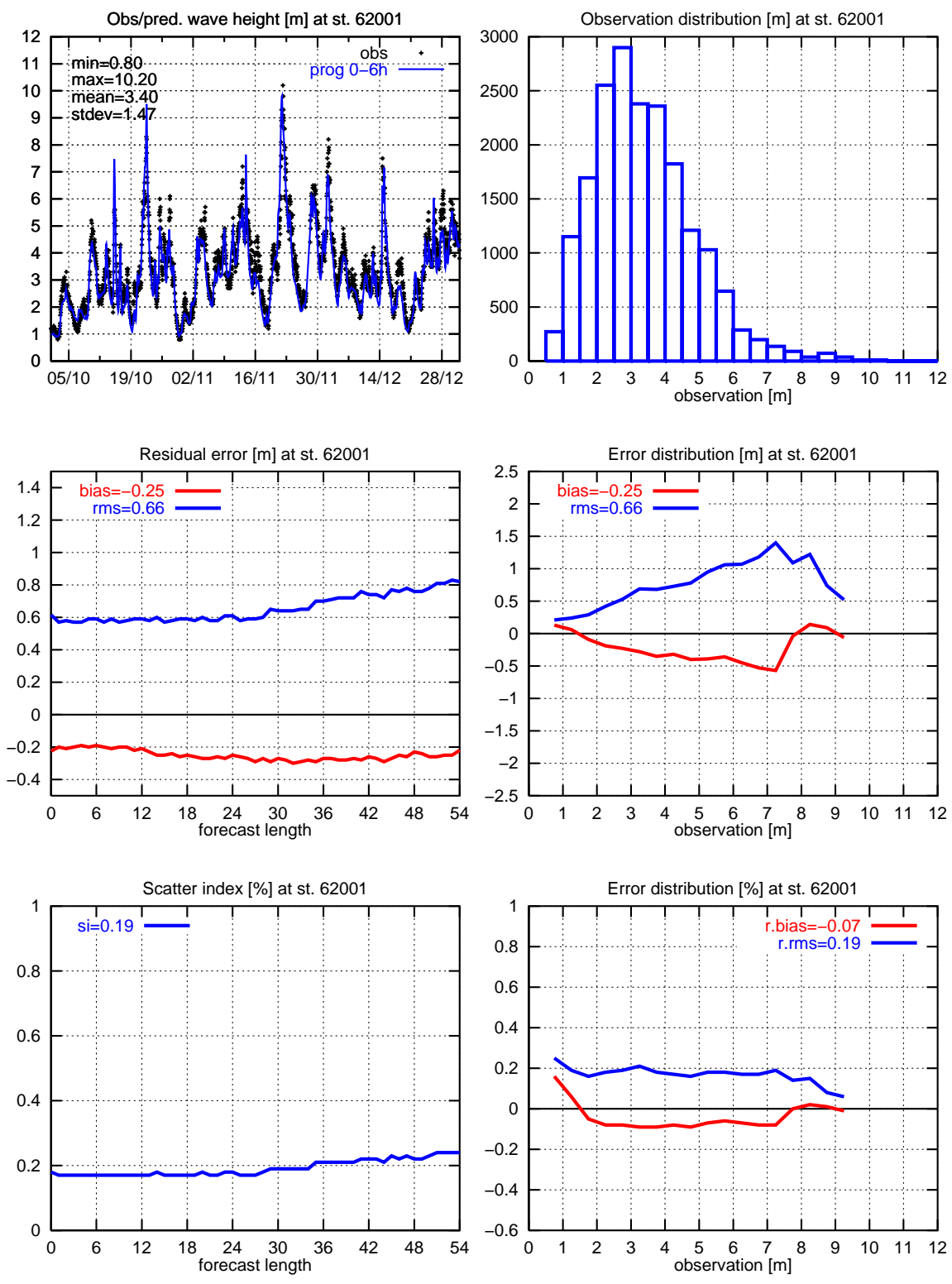
Figure 23. Significant wave height: 62001
