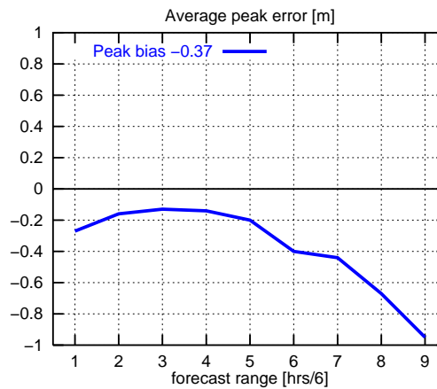
Figure 8. Peak wave height errors.
