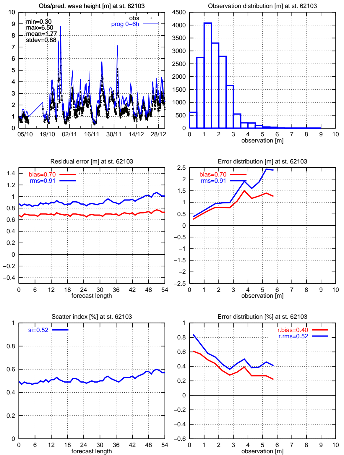
Figure 27. Significant wave height: 62103
