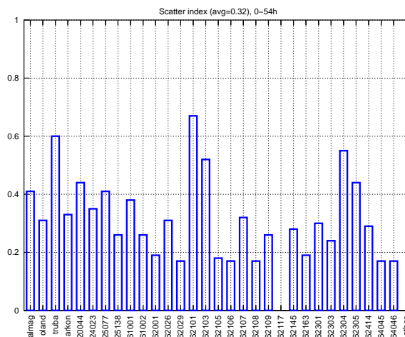
Figure 6. Significant wave height: scatter index. A scatter index of 0.15-0.20 may be considered as a limit due to stochastic processes.
