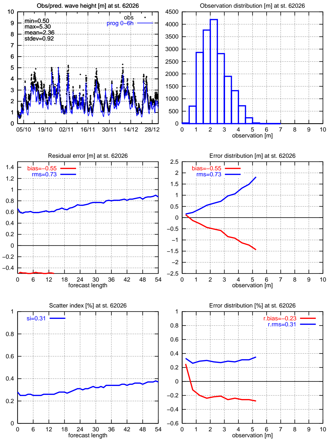
Figure 24. Significant wave height: 62026
