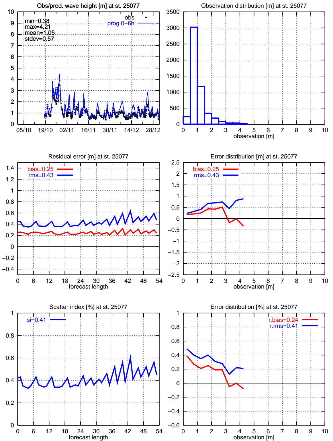
Figure 19. Significant wave height: 25077. The zig-zag curves are caused by irregular 3h sampling.
