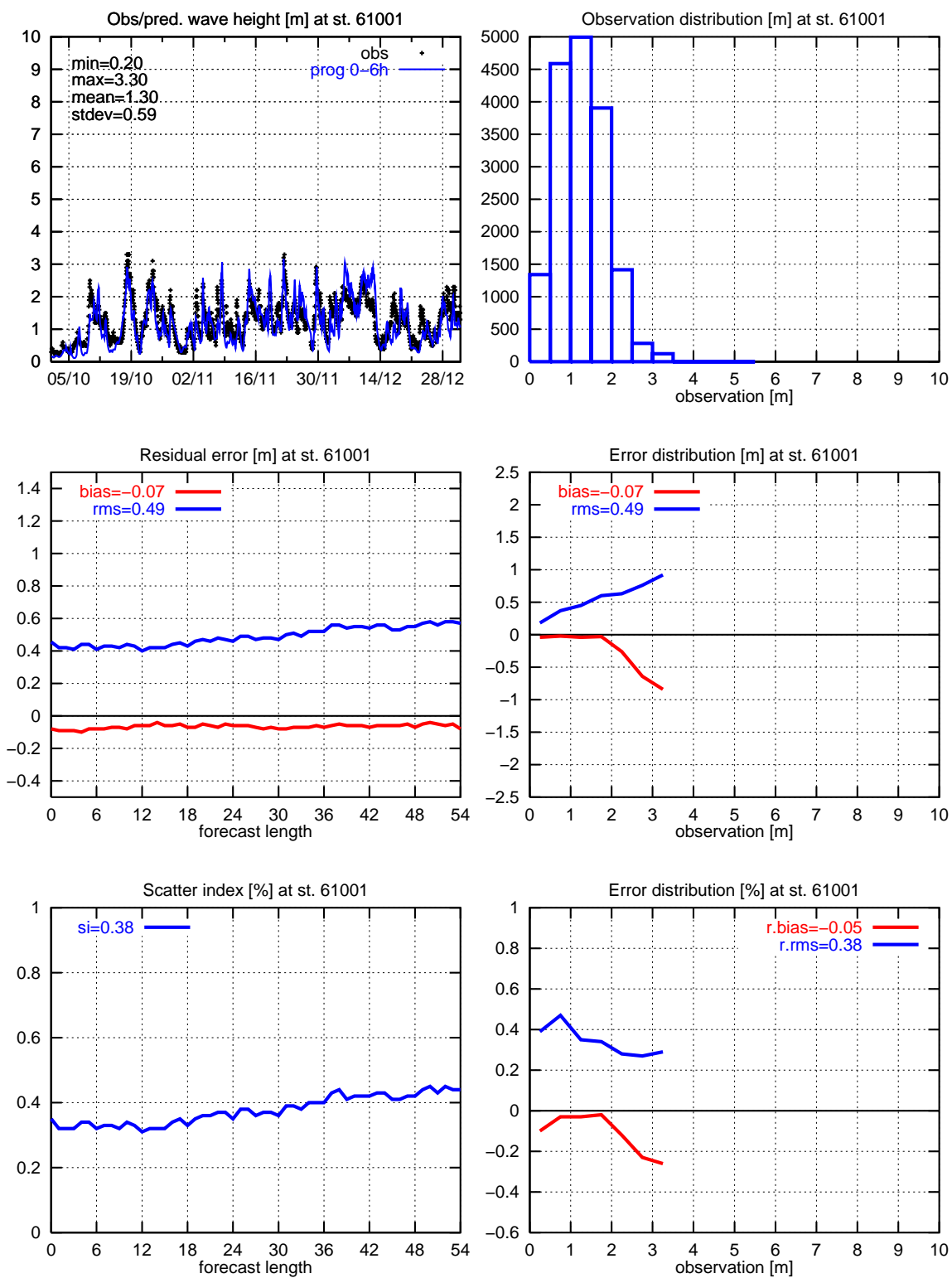
Figure 21. Significant wave height: 61001
