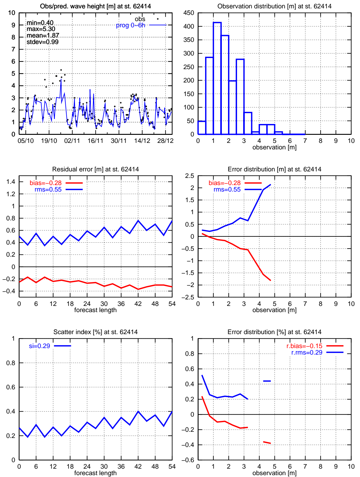
Figure 39. Significant wave height: 62414. The zig-zag curves are caused by irregular 3h sampling.
