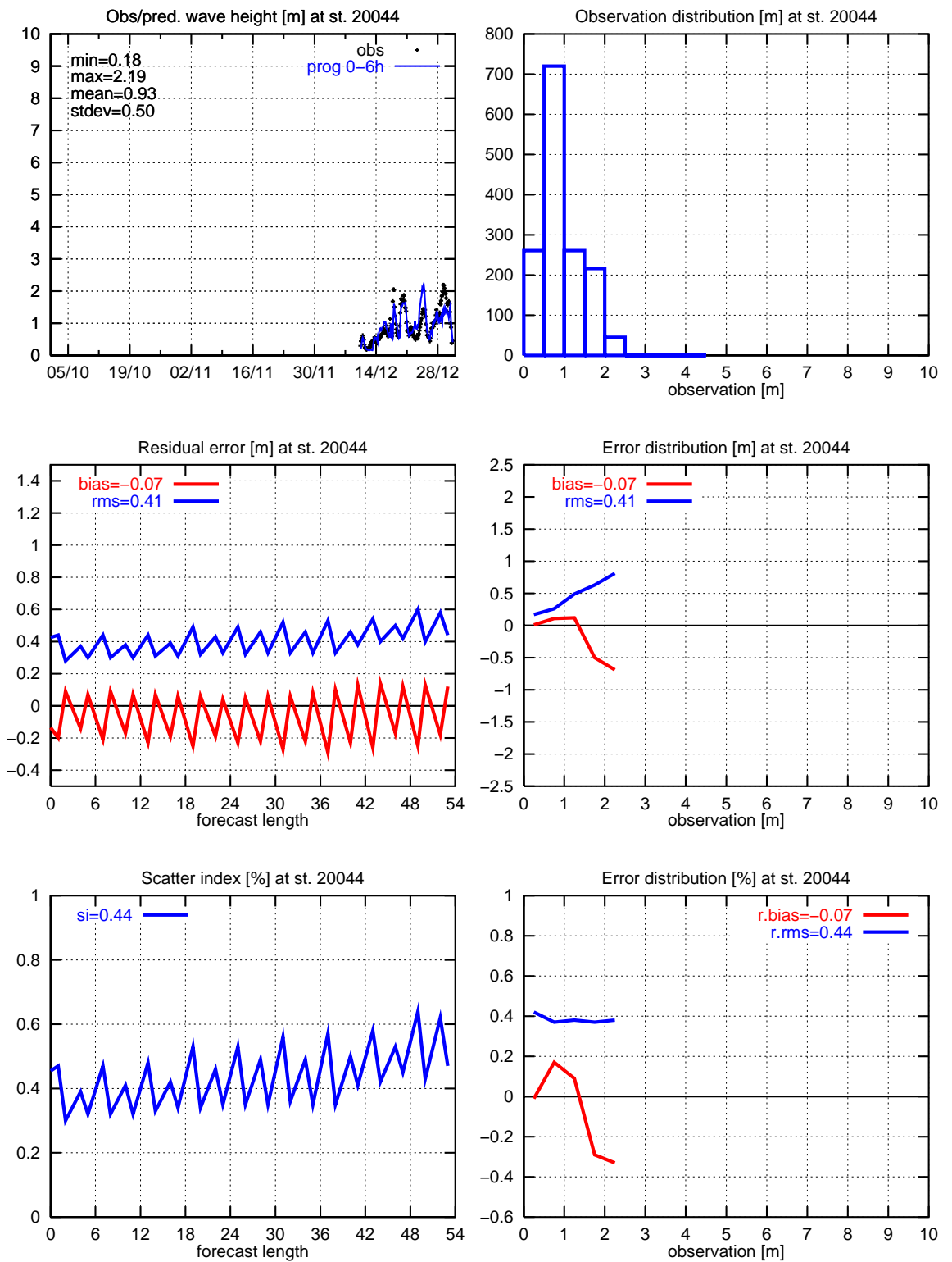
Figure 17. Significant wave height: 20044. The zig-zag curves are caused by irregular 3h sampling.
