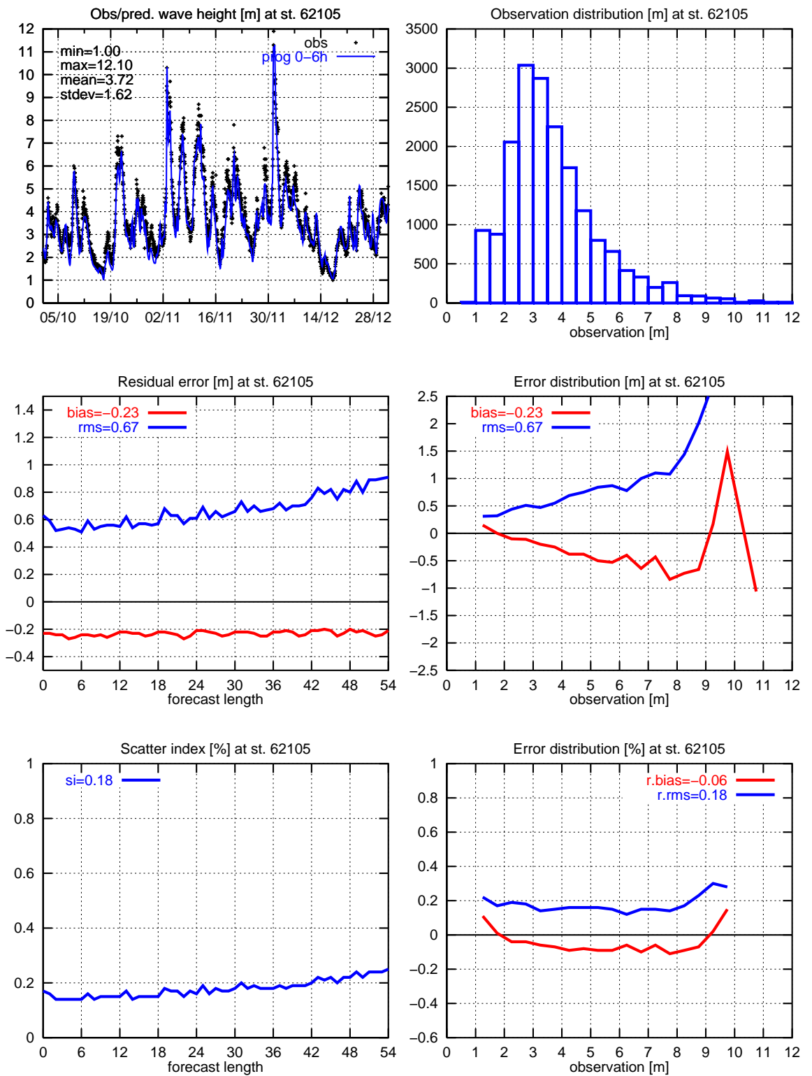
Figure 28. Significant wave height: 62105.
