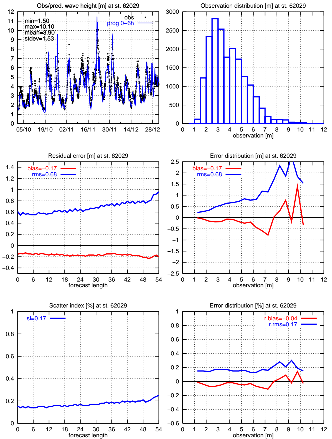
Figure 25. Significant wave height: 62029
