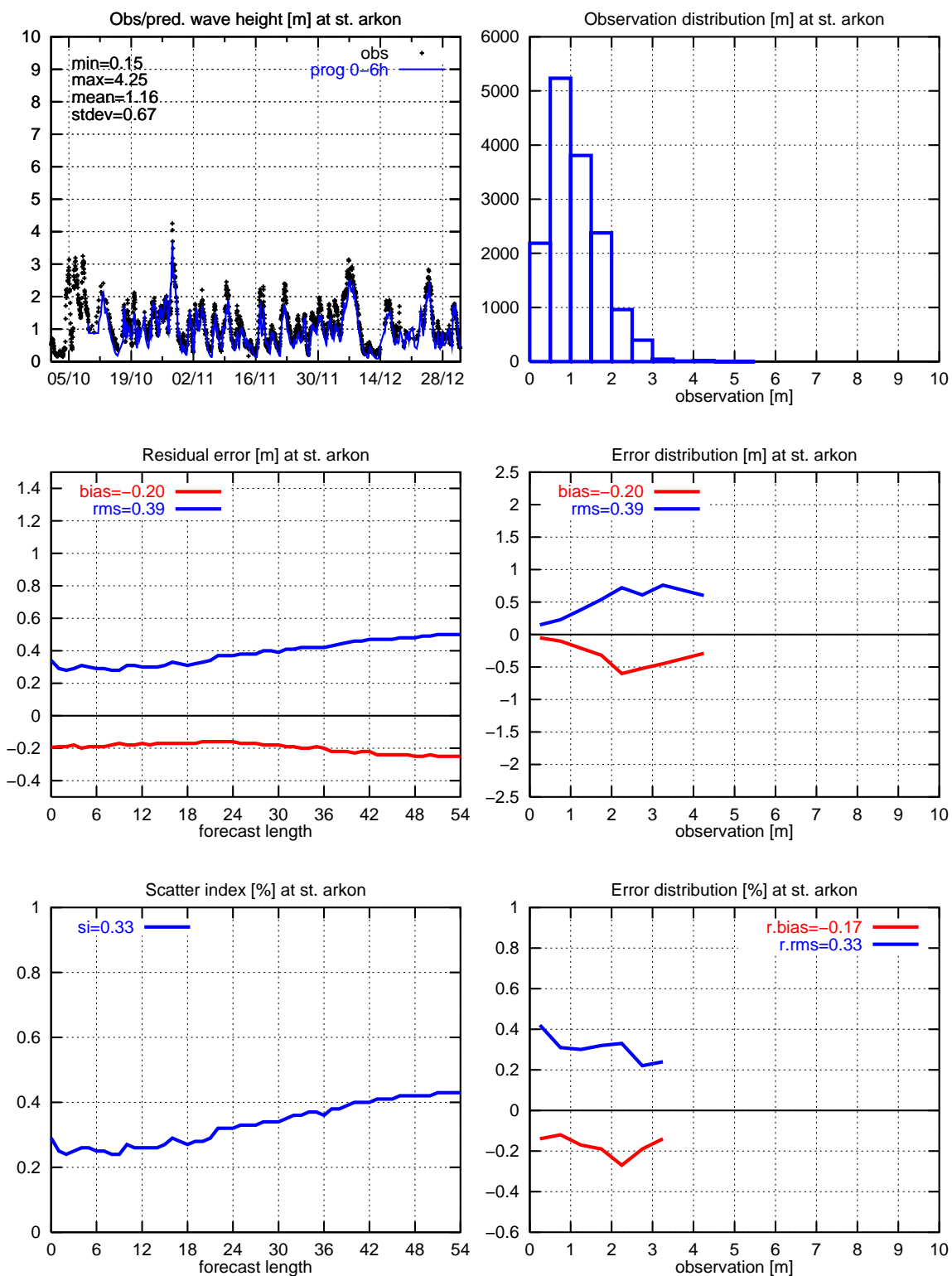
Figure 16. Significant wave height: Arkona
