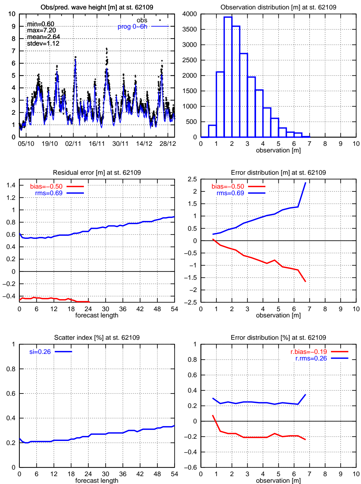
Figure 32. Significant wave height: 62109
