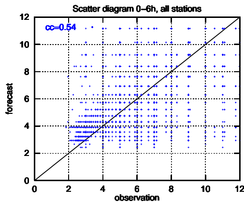
Figure 10. Dominant wave period, 1-6h range.
