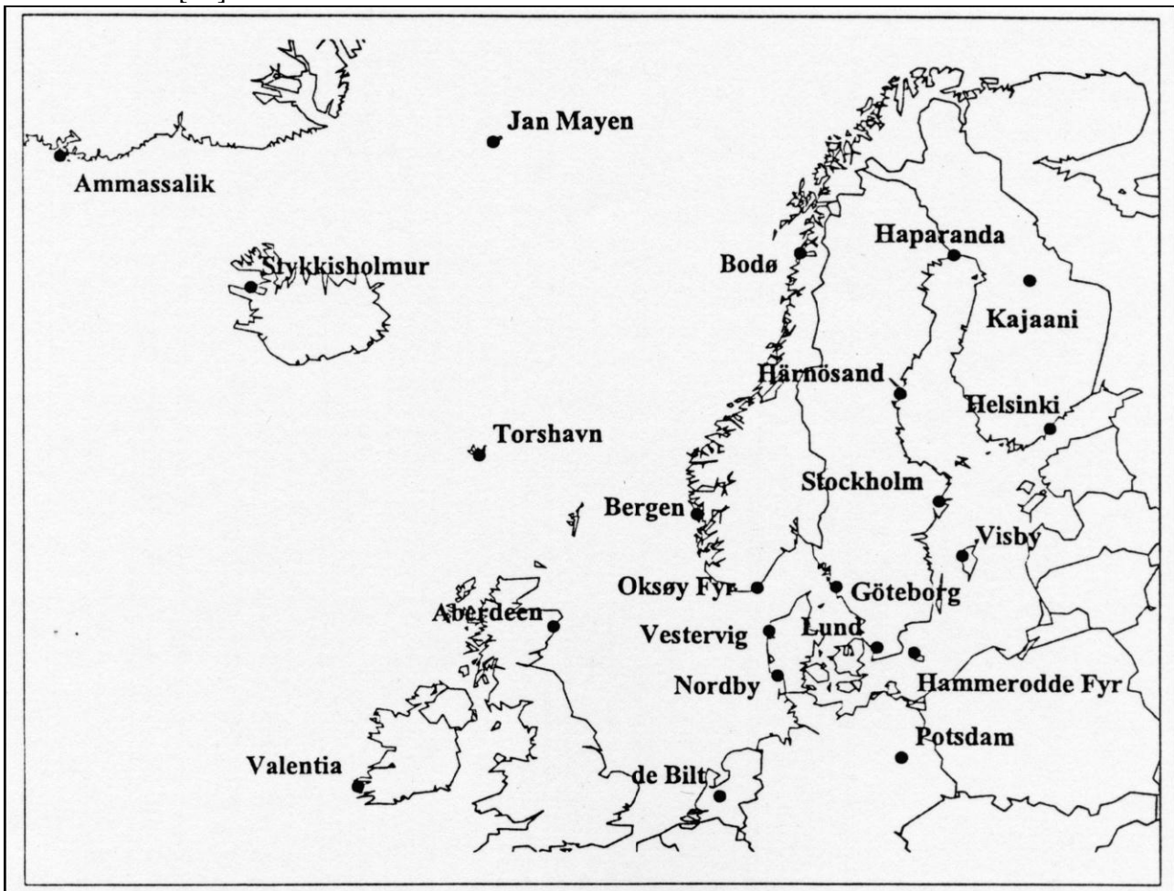
Figure 4.1.1. Location of the stations that originally provided atmospheric pressure observations to the WASA pressure data set [44]. In this report three updated Danish series Hammer Odde Fyr, Nordby and Vestervig are presented. The stations representing these sites are listed in the table 4.2.1. For station co-ordinates confer with the station position file in the data files included in this report (see Appendix 1). Pressure data sets from Tasiilaq/Ammassalik, Greenland and Tórshavn, The Faroe Islands are presented in the representative historical Climate Data Collection; DMI Technical Report 14-04 [23] and DMI Technical Report 14-05 [24].
