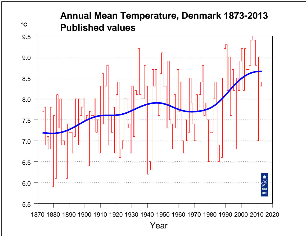
Figure 8.2.3.1. Annual mean temperature, Denmark 1873-2013, published values. A Gauss filter with filter width (standard deviation) 9 years has been used to create the “bold” smooth curve. A Gauss filter with standard deviation 9 years is comparable to a 30-years running mean. However, the filter gives a smoother curve than a running mean, as temperature values from central years are given larger weight than temperature values from periferal years. Filter values are also calculated for the years at either end of the series. It should be noted that these values are computed from one-sided Gauss filters, and that values from later years will change when the series is updated.
