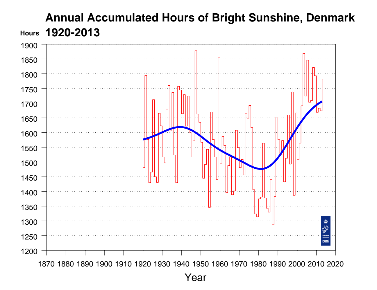
Figure 8.2.3.4. Annual accumulated hours of bright sunshine, Denmark 1920-2013. A Gauss filter with filter width (standard deviation) 9 years has been used to create the “bold” smooth curve. A Gauss filter with standard deviation 9 years is comparable to a 30-years running mean. However, the filter gives a smoother curve than a running mean, as sunshine values from central years are given larger weight than sunshine values from periferal years. Filter values are also calculated for the years at either end of the series. It should be noted that these values are computed from one-sided Gauss filters, and that values from later years will change when the series is updated.
