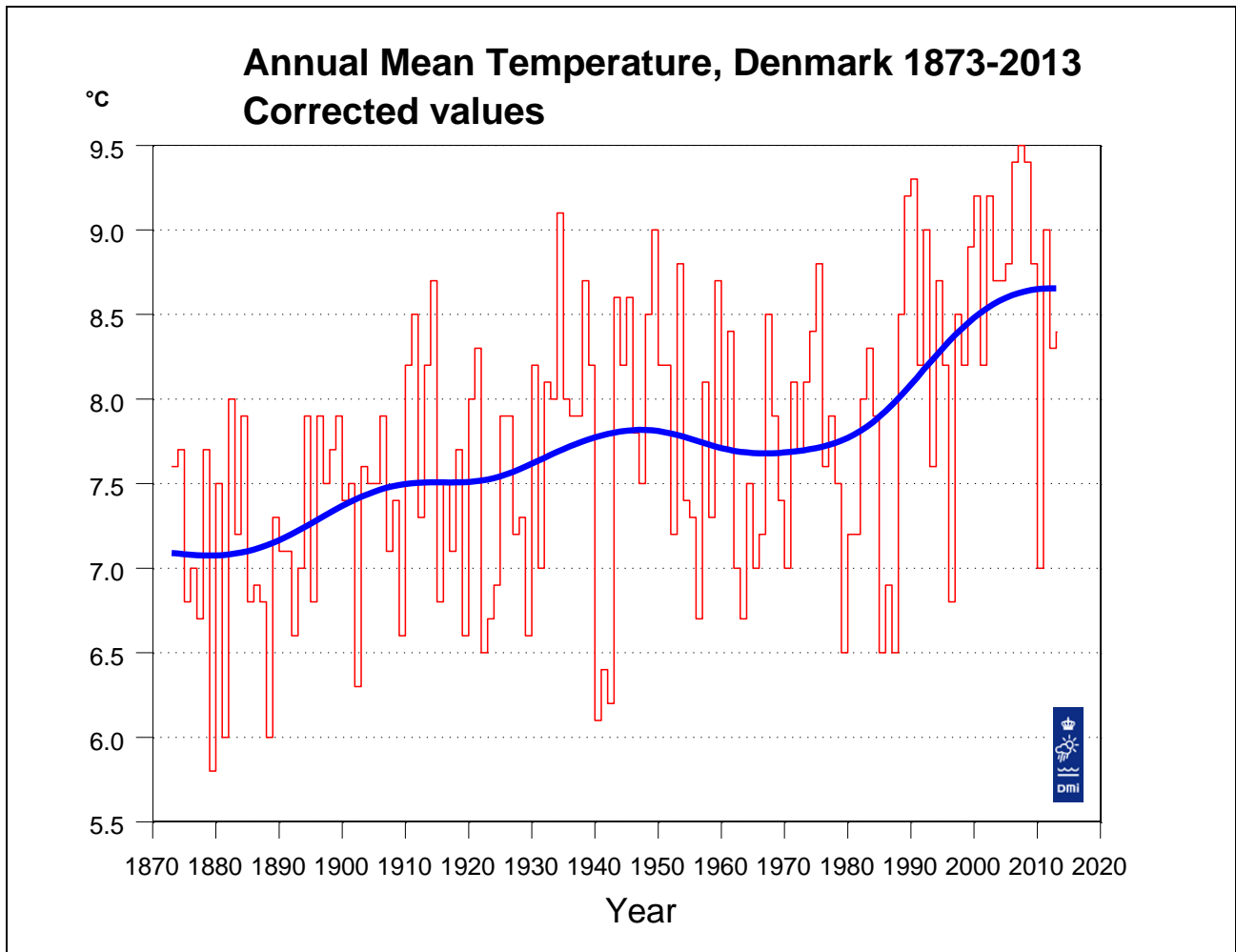
Figure 8.2.3.2. Annual mean temperature, Denmark 1873-2013, corrected values. A Gauss filter with filter width (standard deviation) 9 years has been used to create the “bold” smooth curve. A Gauss filter with standard deviation 9 years is comparable to a 30-years running mean. However, the filter gives a smoother curve than a running mean, as temperature values from central years are given larger weight than temperature values from periferal years. Filter values are also calculated for the years at either end of the series. It should be noted that these values are computed from one-sided Gauss filters, and that values from later years will change when the series is updated.
