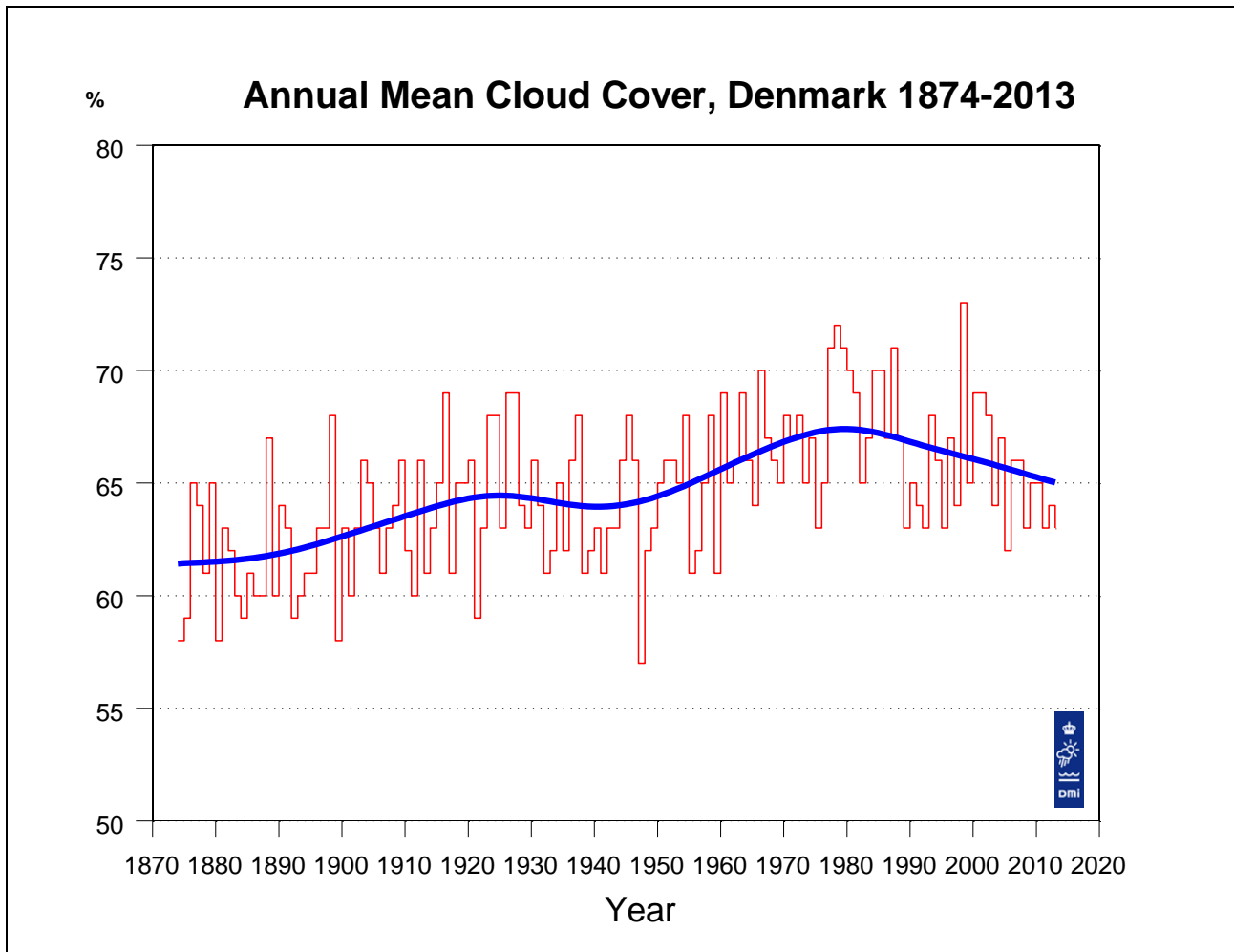
Figure 8.2.3.5. Annual mean cloud cover, Denmark 1874-2013. The annual value is calculated using manually observed cloud cover data from seven manned stations at airports. A Gauss filter with filter width (standard deviation) 9 years has been used to create the “bold” smooth curve. A Gauss filter with standard deviation 9 years is comparable to a 30-years running mean. However, the filter gives a smoother curve than a running mean, as cloud cover values from central years are given larger weight than cloud cover values from periferal years. Filter values are also calculated for the years at either end of the series. It should be noted that these values are computed from one-sided Gauss filters, and that values from later years will change when the series is updated.
