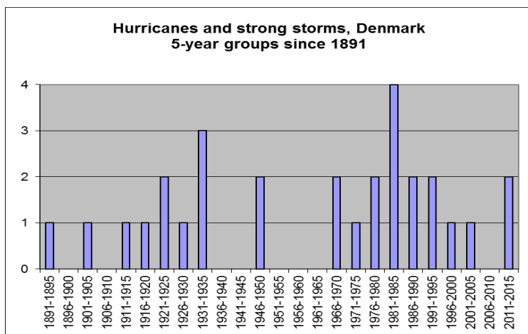
Class 3 and 4 storms in 5-year groups since 1891.
